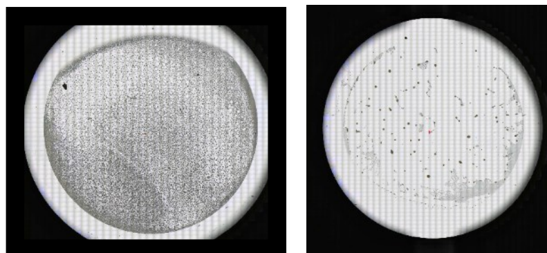
Figure 3-21: optical mosaic of the 2021 residues Sd7 (left) and Sd8 (right) on the 20 mm large Si substrate windows. Sd7 residue has the characteristic shape of residue obtained with N_2 -dominated ices with a homogeneous structure on the substrate window. Sd8 residue is the one obtained with NH_3 -dominated ice, the matter is concentrated around smaller spots but much thicker, up to 5\ \mu m in height.
