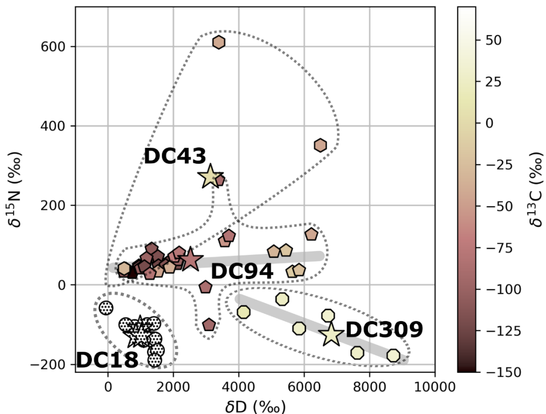
Figure 2-27: summary of the \delta\text{D} , \delta^{15}\text{N} and \delta^{13}\text{C} measured on DC309, DC18, DC43 and DC94. The color scale indicates the \delta^{13}\text{C} values. Bulk composition are plotted with stars and measurements on ROIs by circles (DC18), octagons (DC309), hexagons (DC43) and pentagons (DC94). The linear correlations observed in DC309 and DC94 are represented by gray thick lines.
