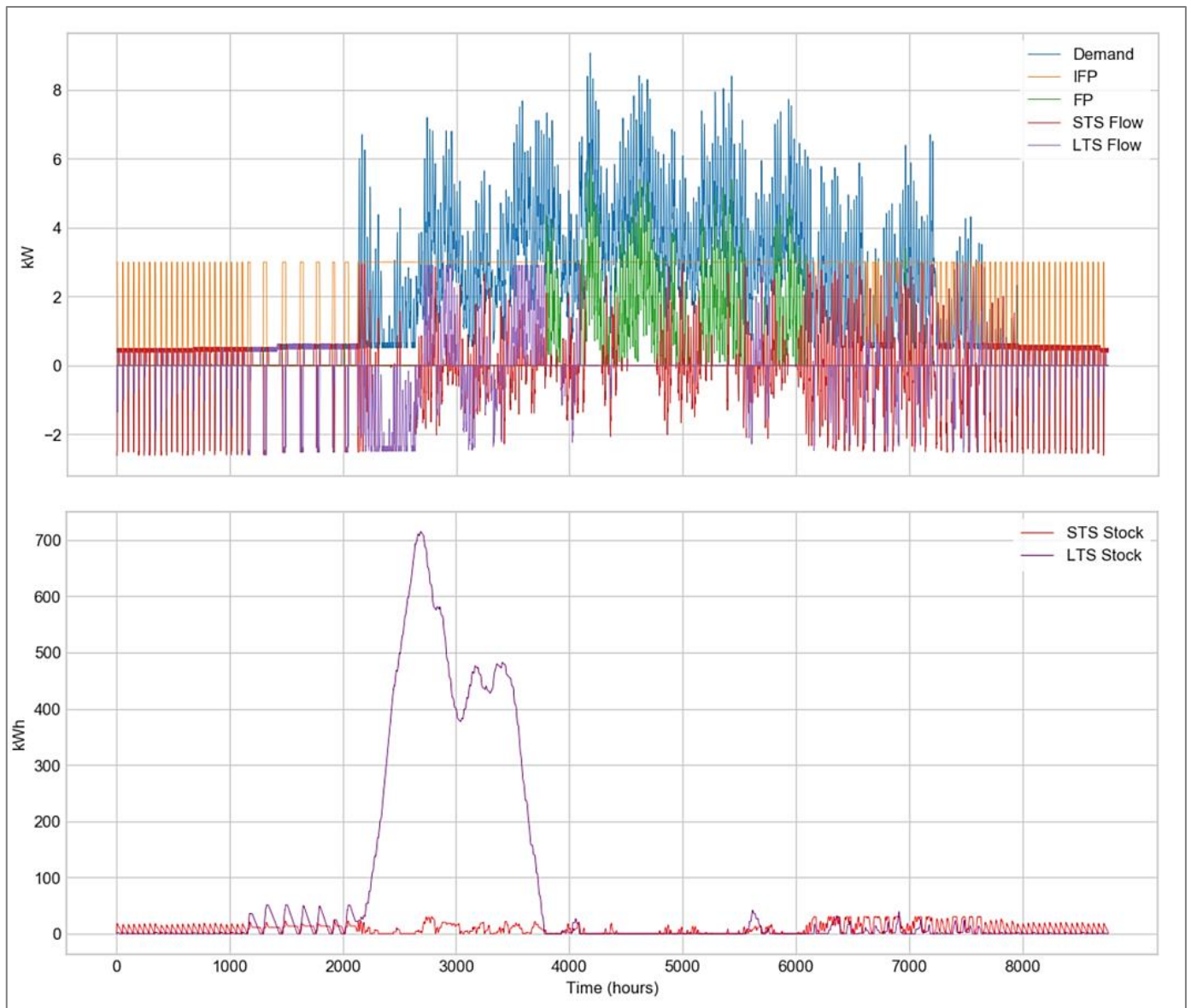
Figure 19: Results for the RpCf model, with horizon H1.
