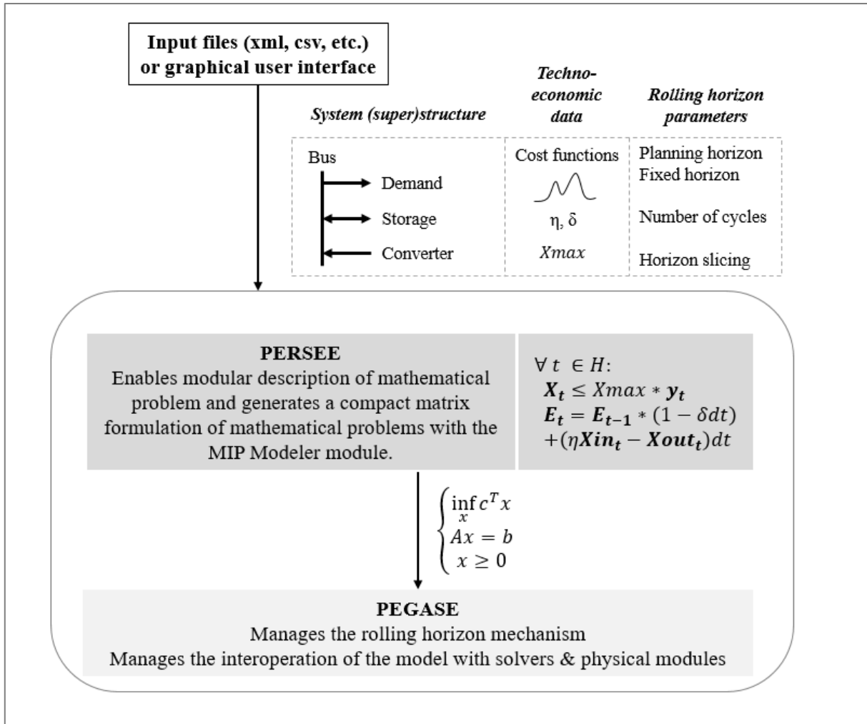
Figure 13: Schematic description of the modelling environment
