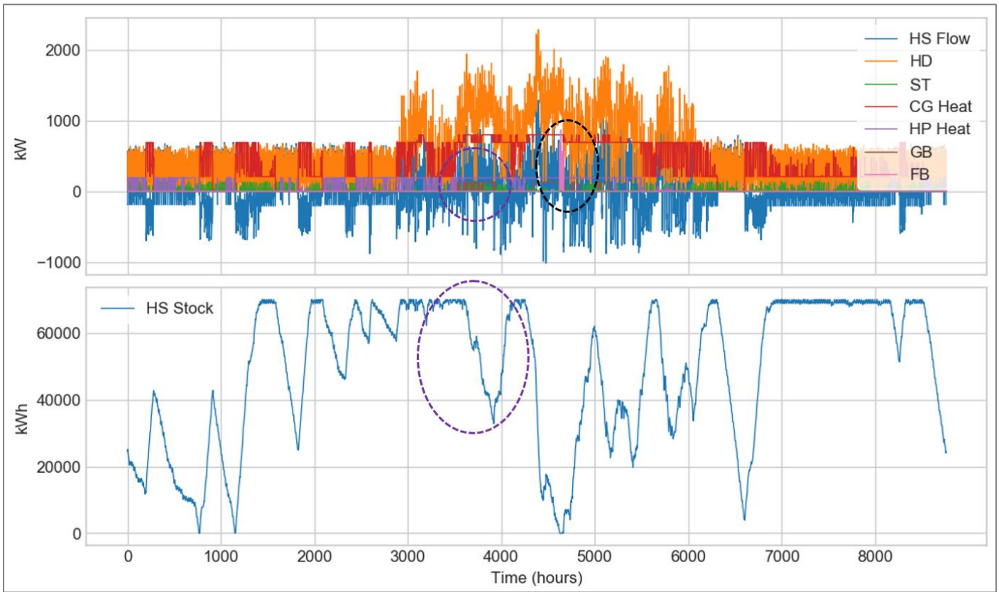
Figure 52: Heat power balance for the MILP-RpCfH3 configuration, case where the HD is overestimated by 20% after 24h.
