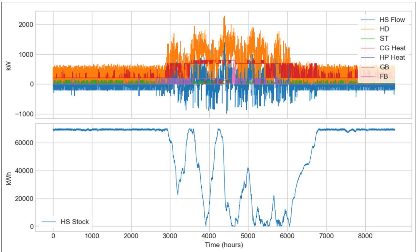
Figure 49: Heat power and balance and storage state for the MILP-MeanH2 configuration.
