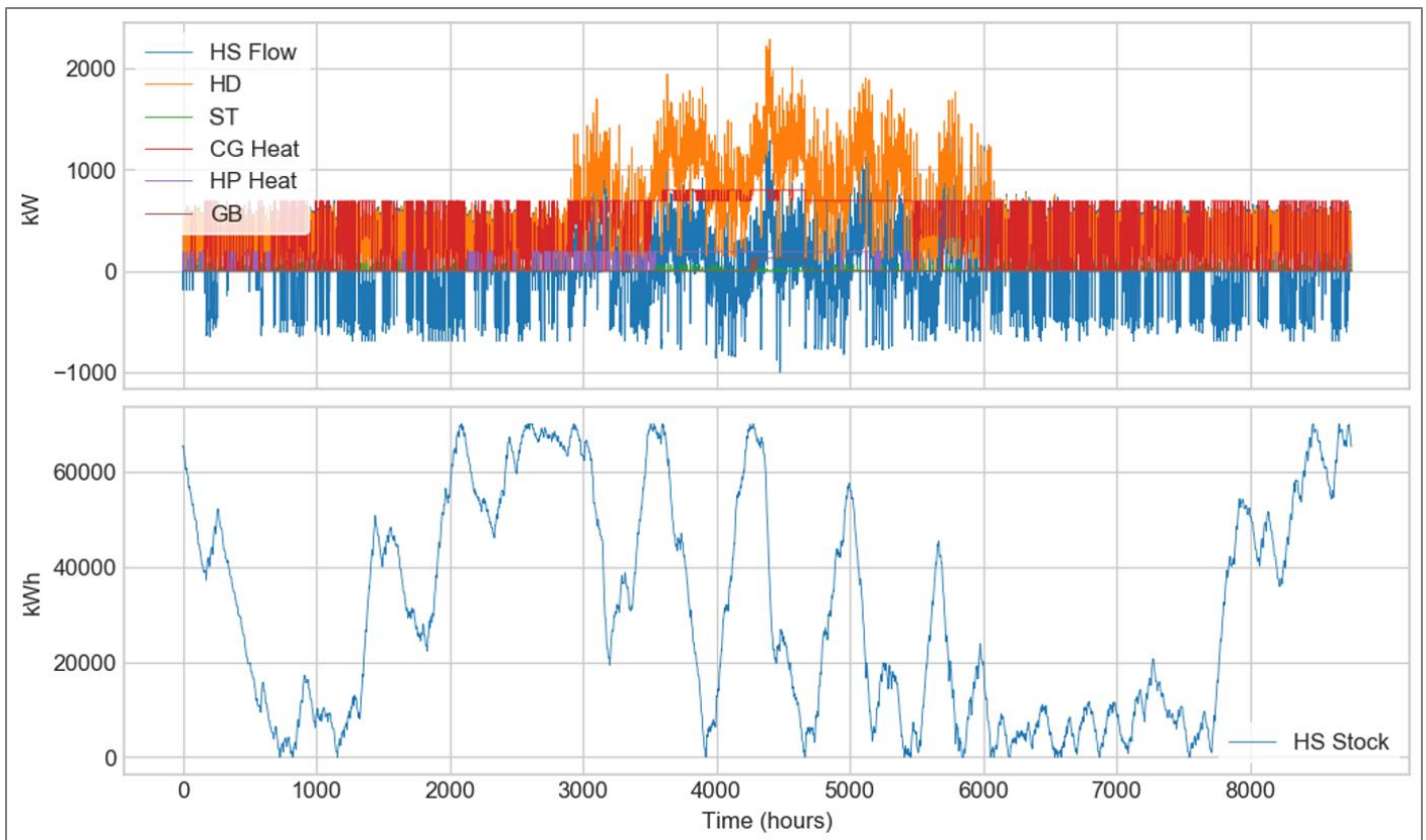
Figure 38: Solution of the OneShot-LP configuration: heat power balance and HS state
