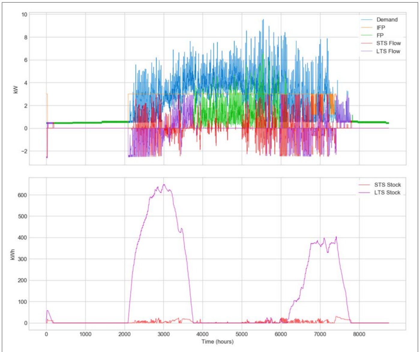
Figure 22: Solution of the RpCf-SetUp model in case where the FP cost is 44.4 euros and the demand profile B is considered..
