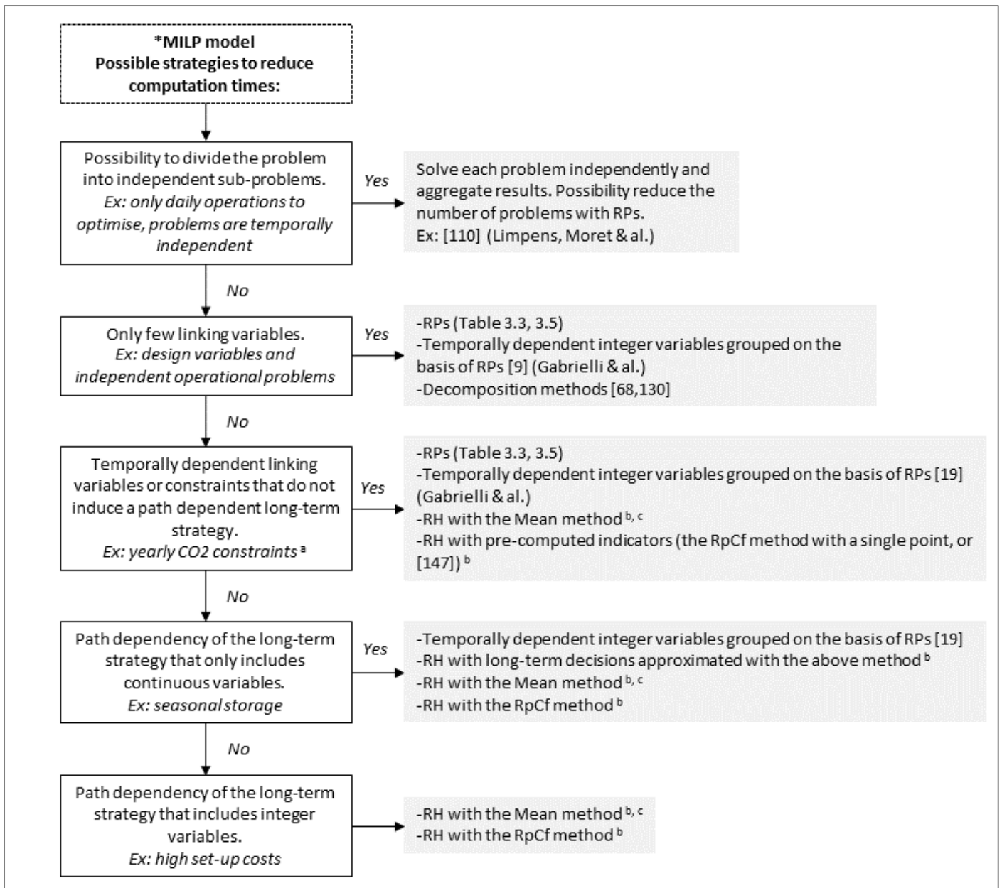
Figure 54: Options to reduce computation times, according to the problem structure
