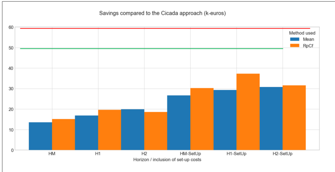
Figure 14: Savings of all approaches compared to the Cicada approach (k-euros), with upper bound (red) and lower bound (green) of the One Shot optimisation.
