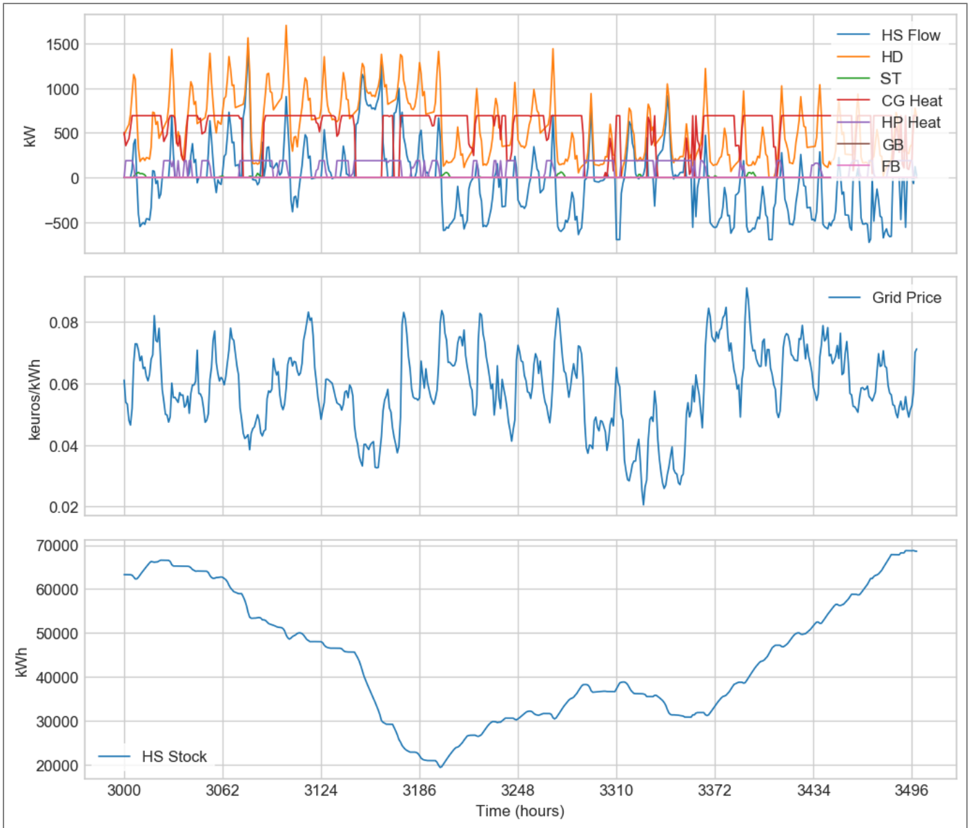
Figure 63: Zoom on the inter-season period, for the LP-OneShot configuration
