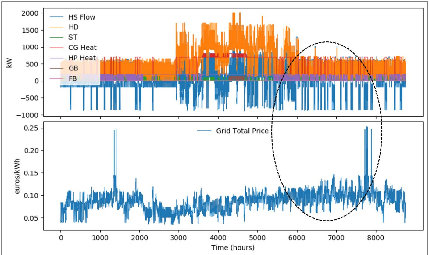
Figure 41: Solution of the OneShot-MILP-RP configuration when 48 RPs of 2 days are used: heat power balance and grid prices
