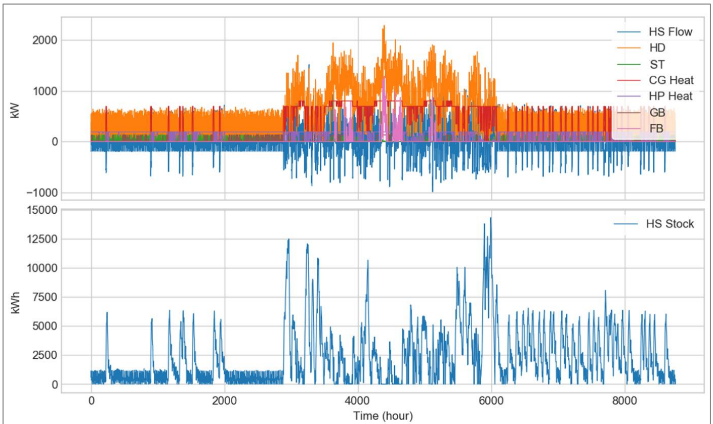
Figure 47: Heat power and balance and storage state for the MILP-Cicada configuration.
