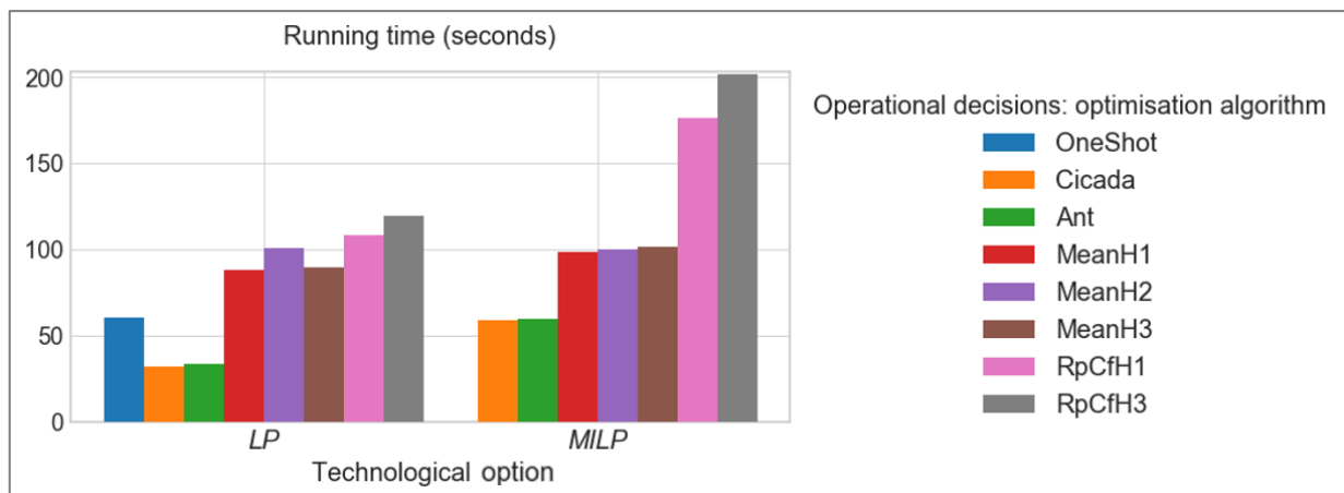
Figure 46: Computation times (time to simulate a year) of the different operational decisions modelling options, for both LP and MILP options. The time limit of one hour was reached with the MILP-OneShot configuration.
