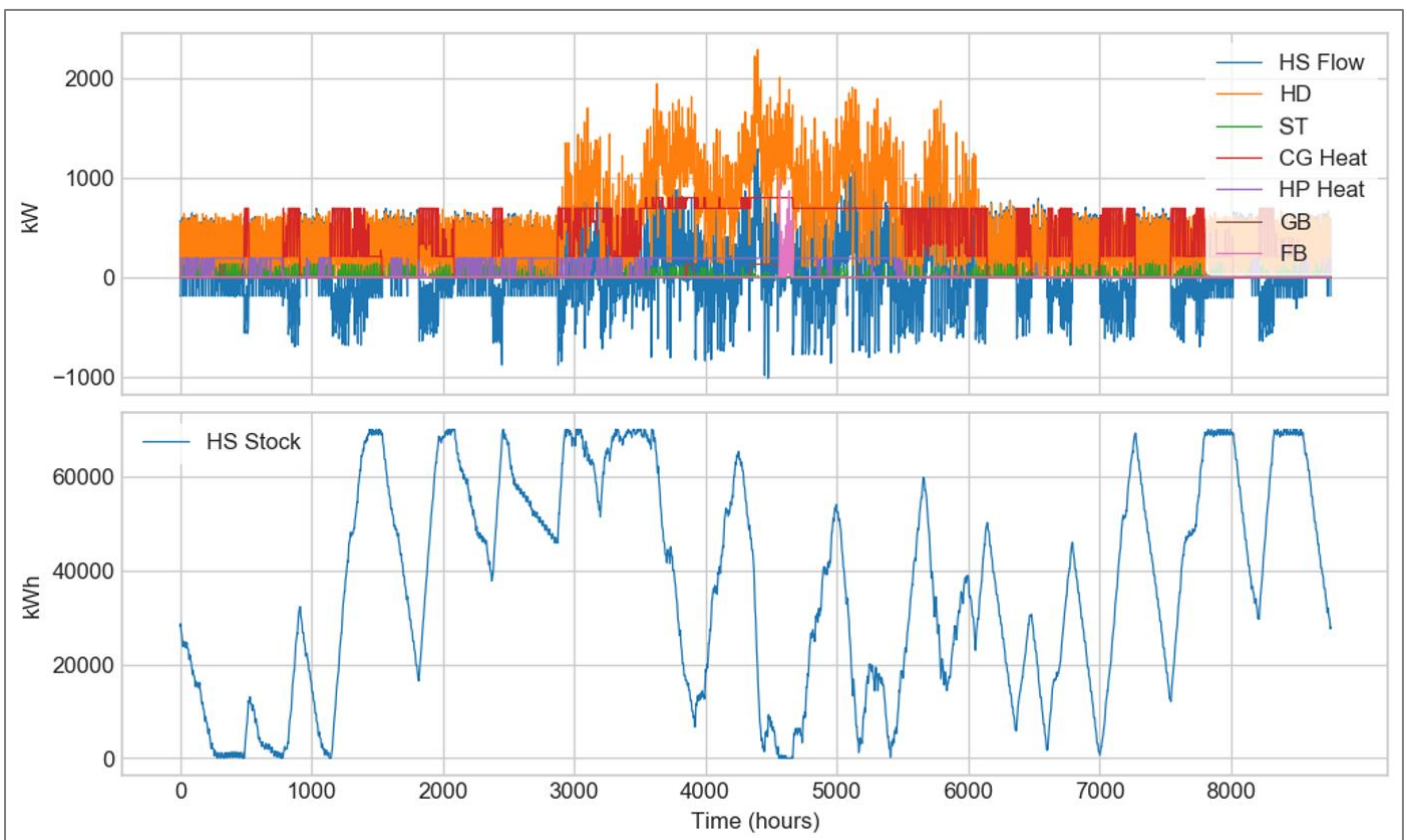
Figure 50: Heat power balance and storage state for the MILP-RpCfH3 configuration.
