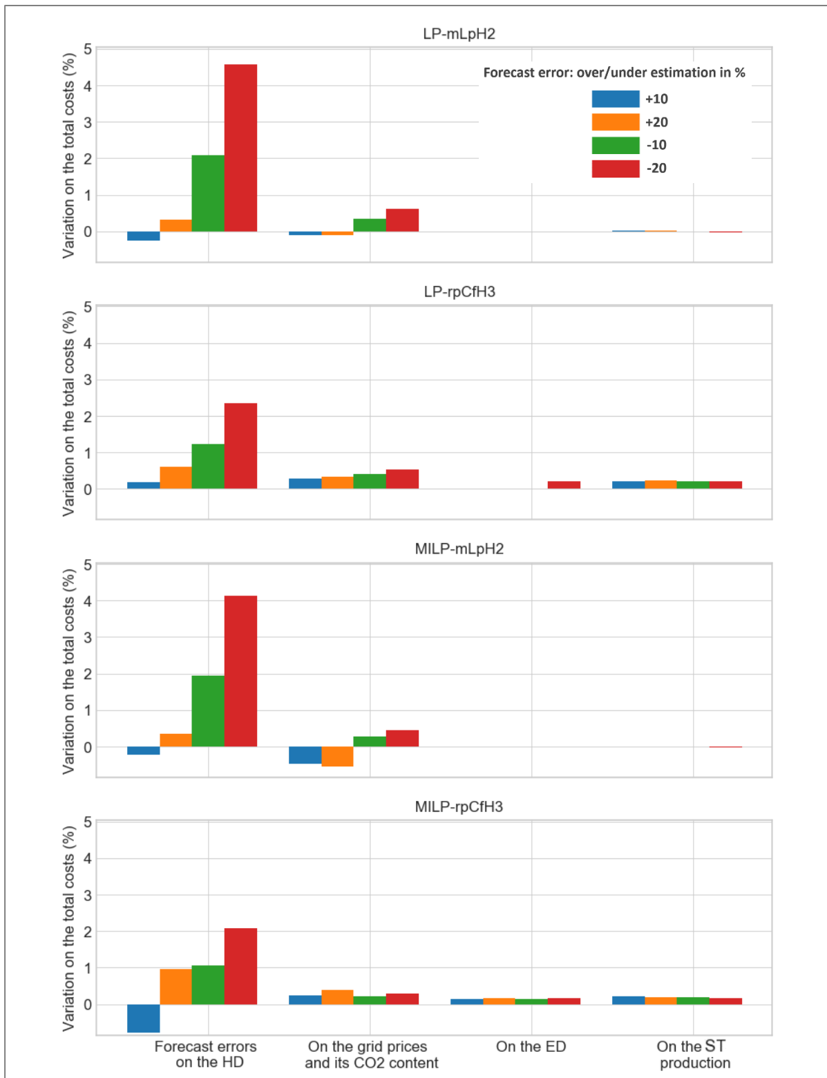
Figure 51: Impact of the forecast assumptions.
