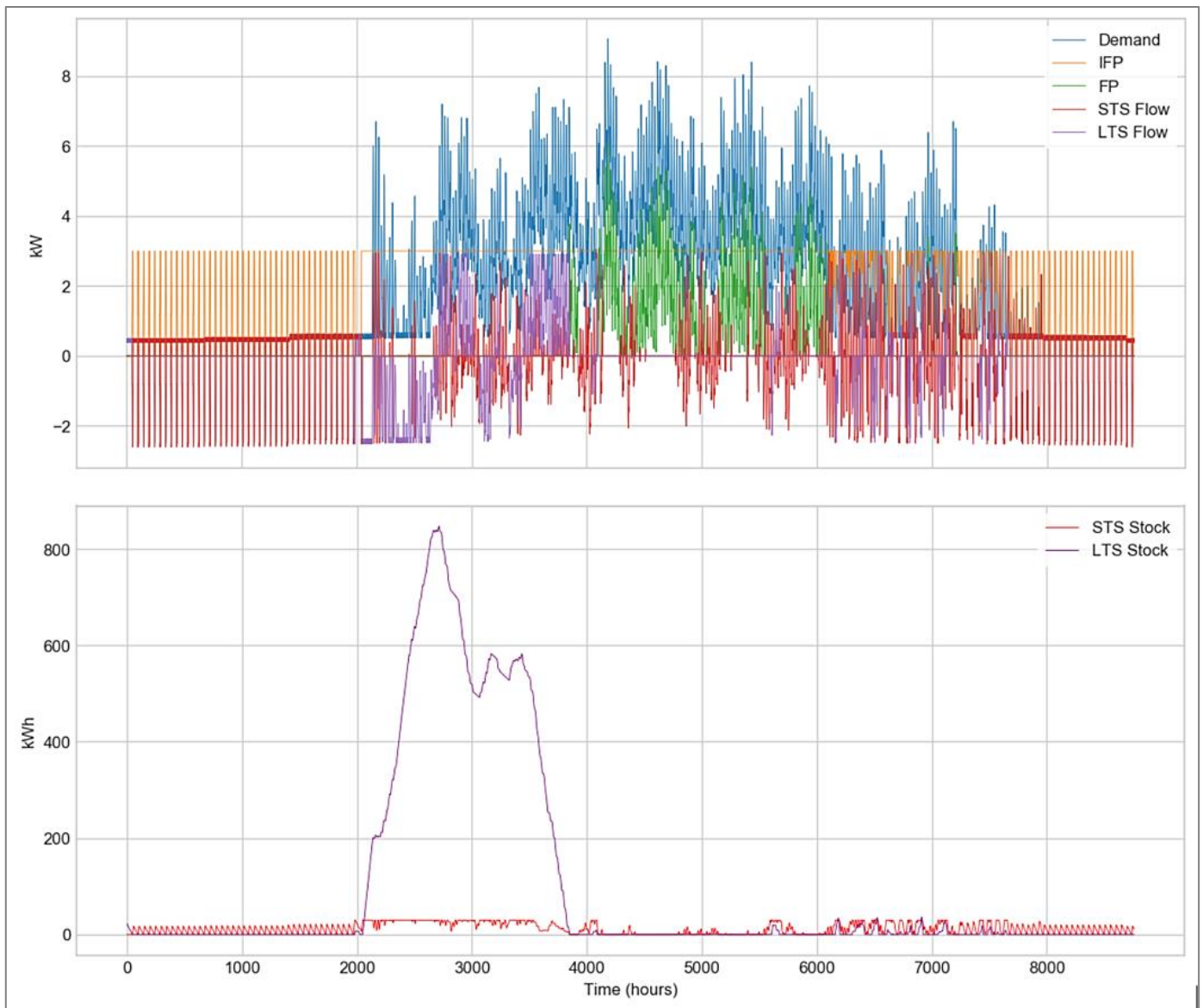
Figure 17: Results for the Mean model, with horizon H1.
