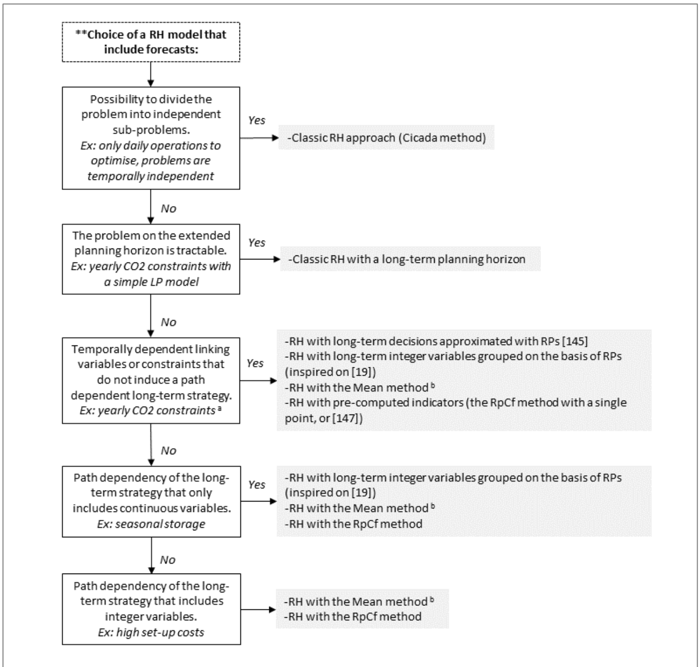
Figure 55: RH horizon methods, according to the problem structure
