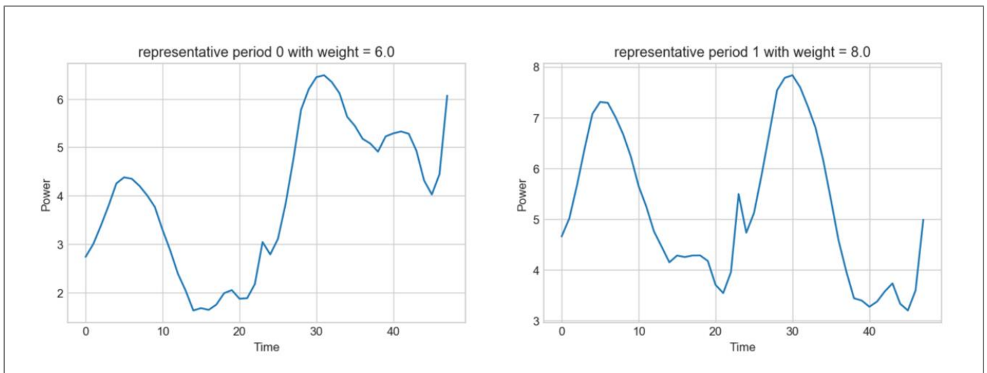
Figure 57: Two RPs of two days for the original data
