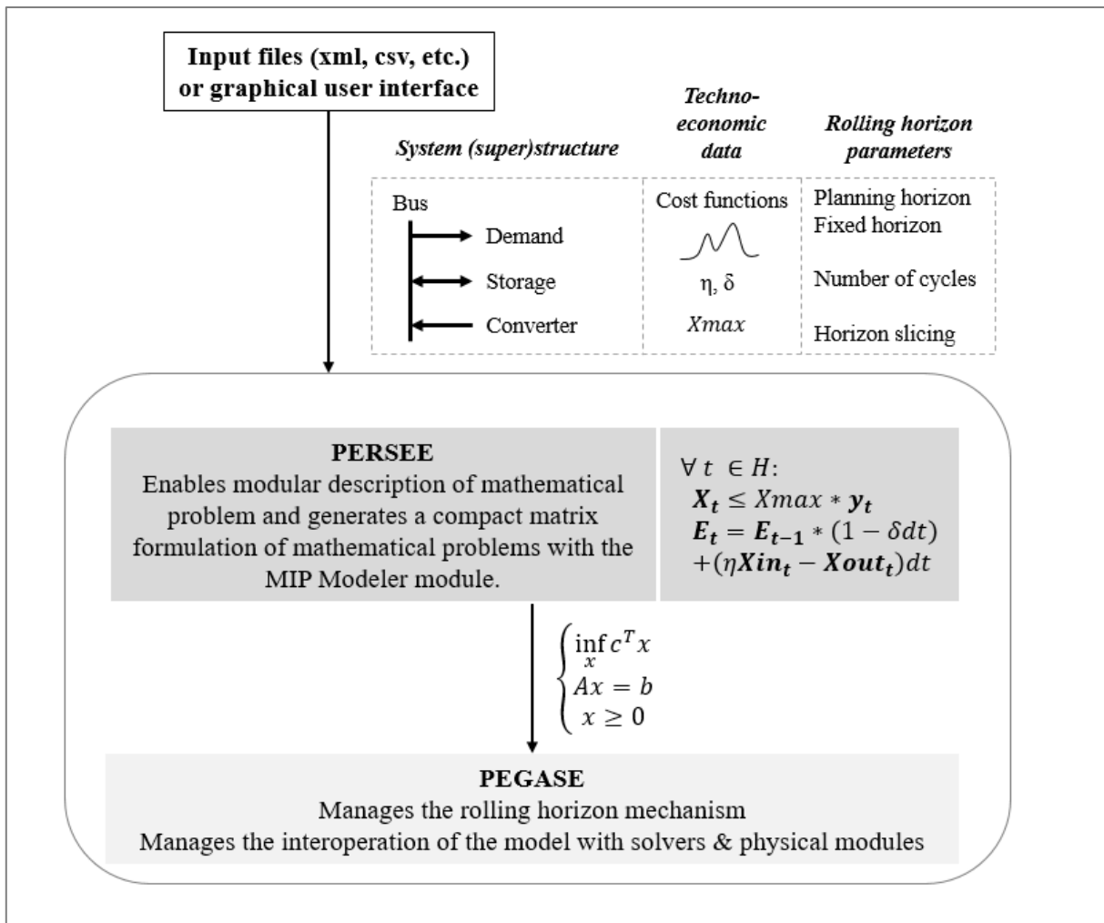
Figure 13: Schematic description of the modelling environment
