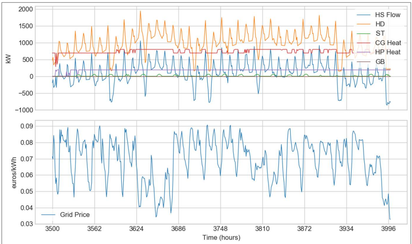
Figure 62: Zoom on the winter period, the strategy is identical for the LP-OneShot and the MILP-OneShot configurations
