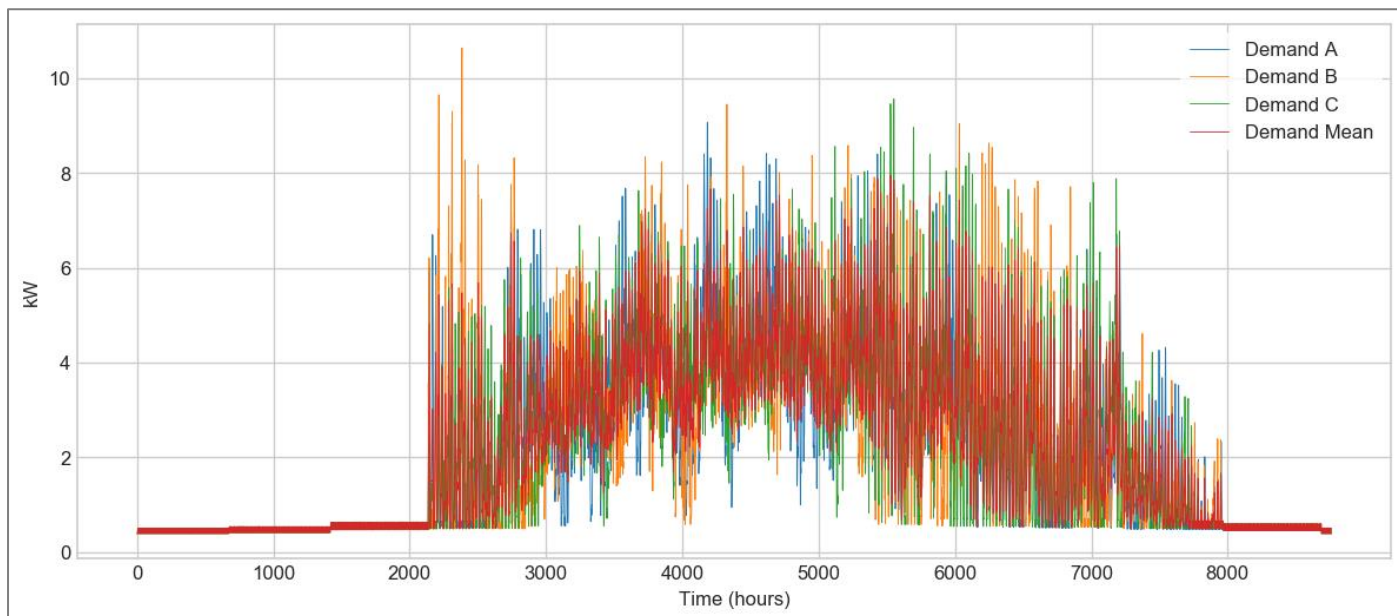
Figure 60: Demand profiles.
