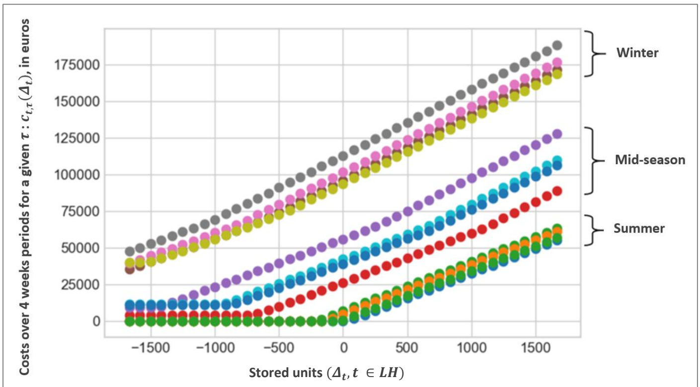
Figure 59: Computed cost functions.
