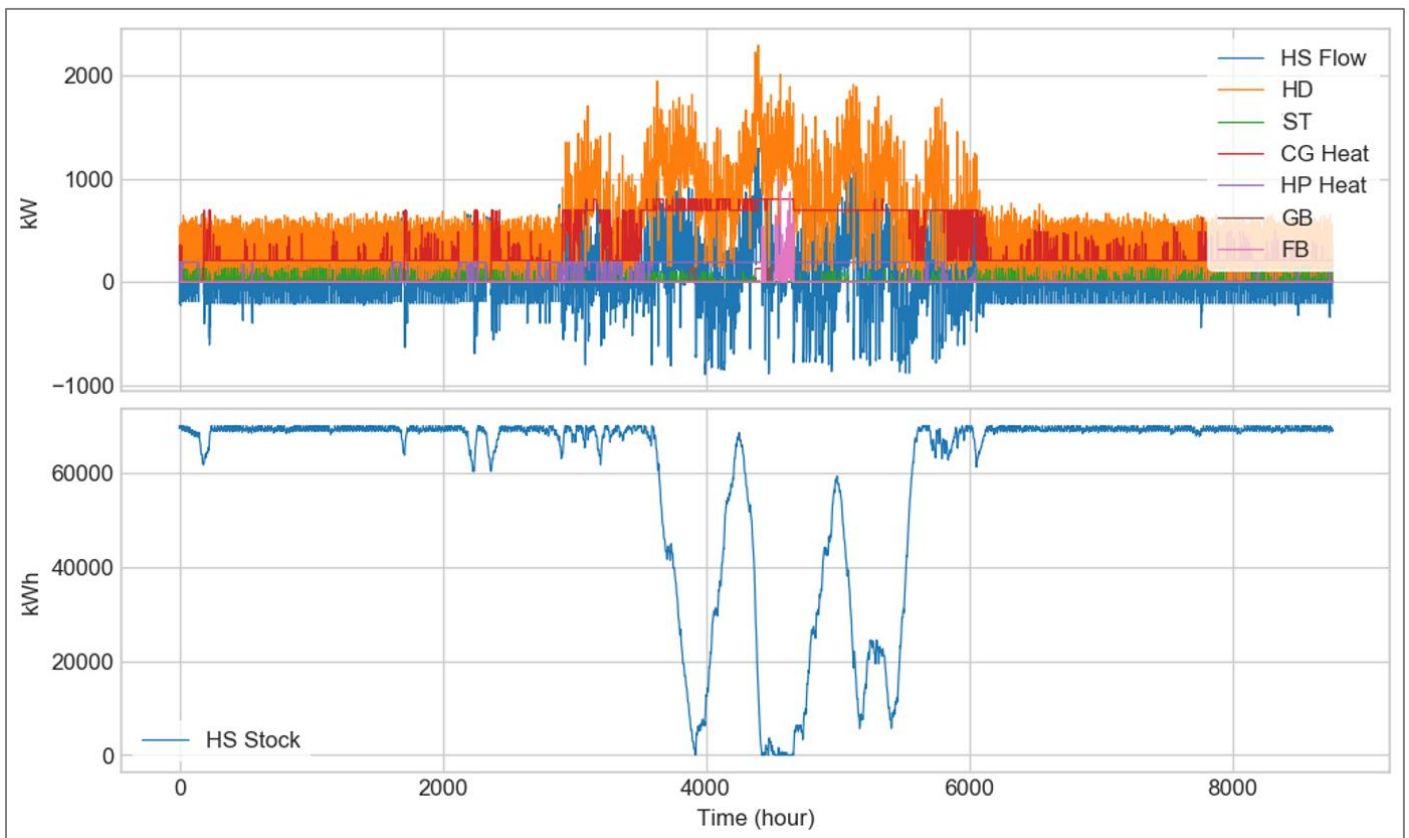
Figure 48: Heat power and balance and storage state for the MILP-Ant configuration.
