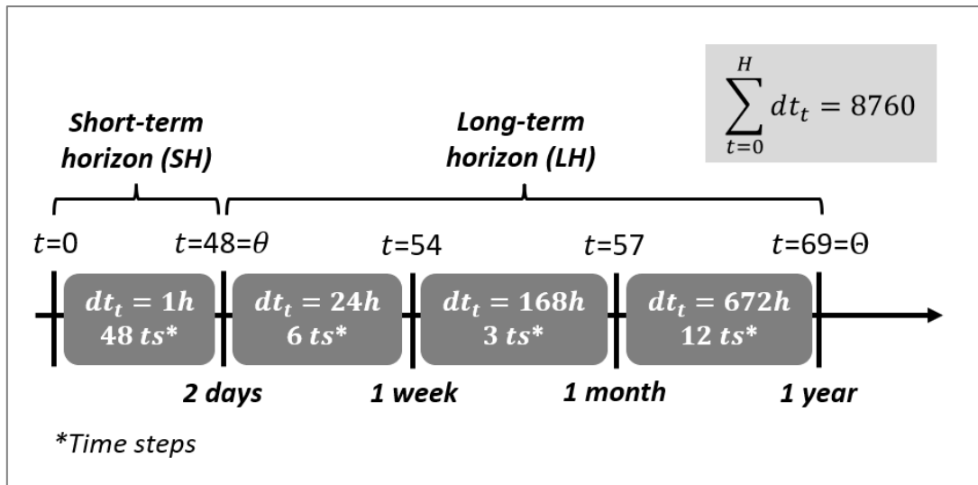
Figure 10: Planning horizon including a long-term vision with aggregated time steps
