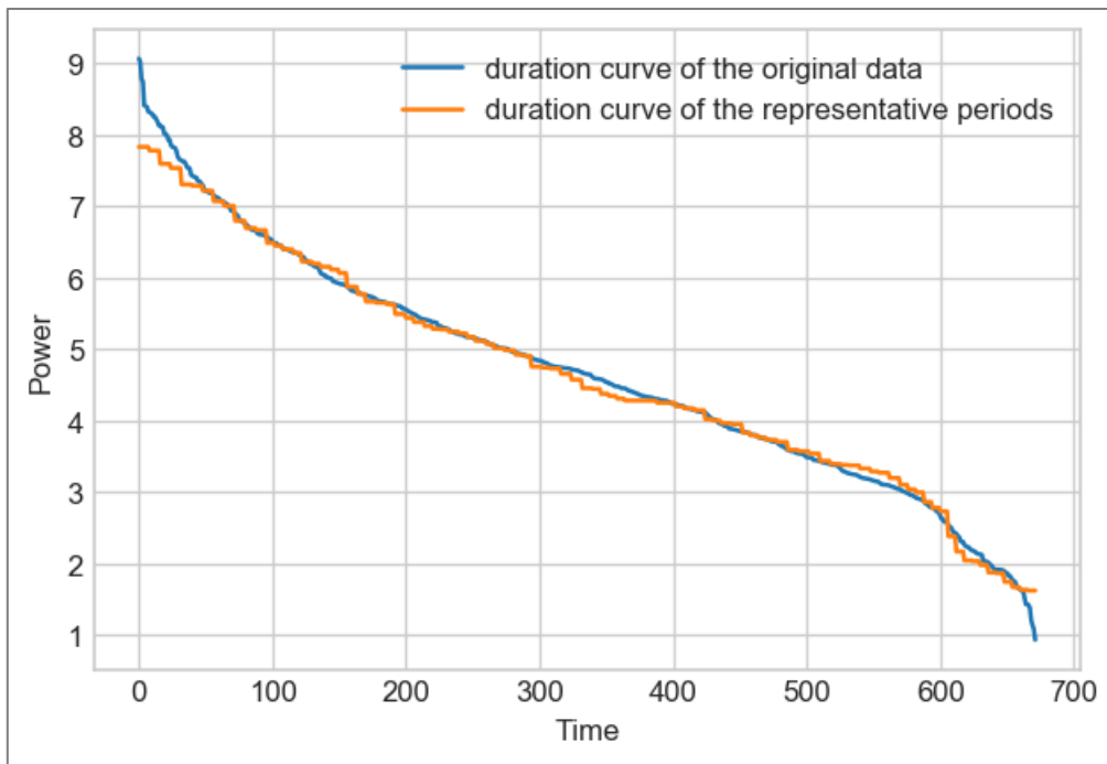
Figure 58: Corresponding duration curves for both original RPs, the method minimises the difference between both curves.
