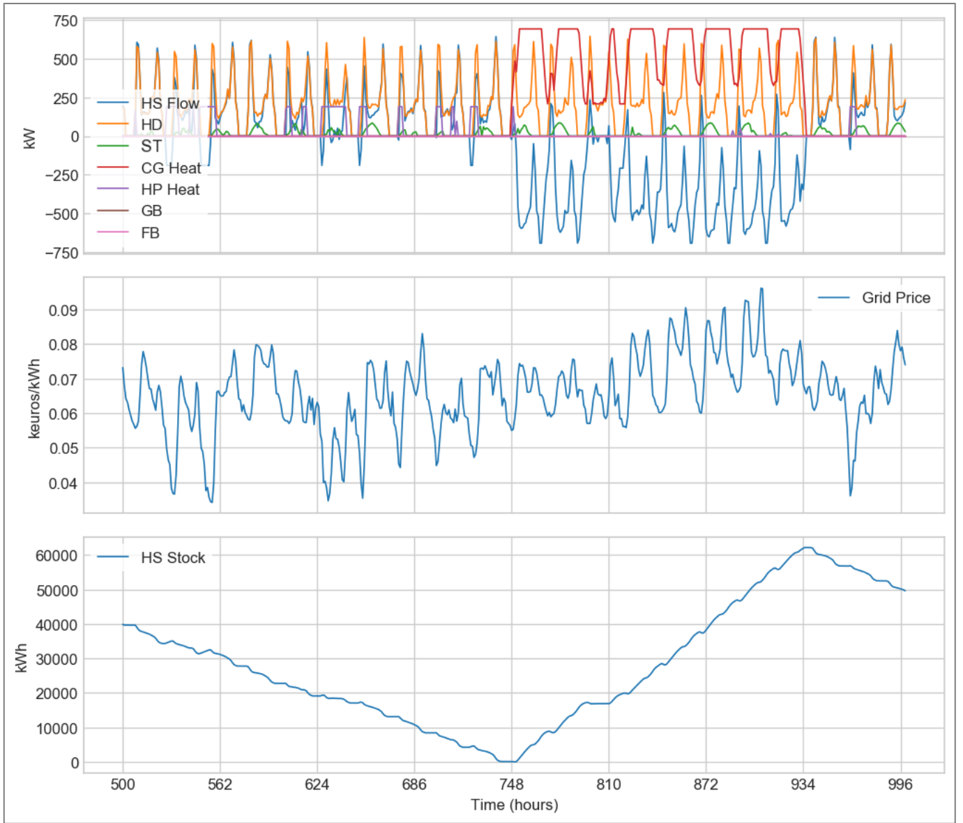
Figure 66: Zoom on the inter-season period, for the MILP-OneShot configuration
