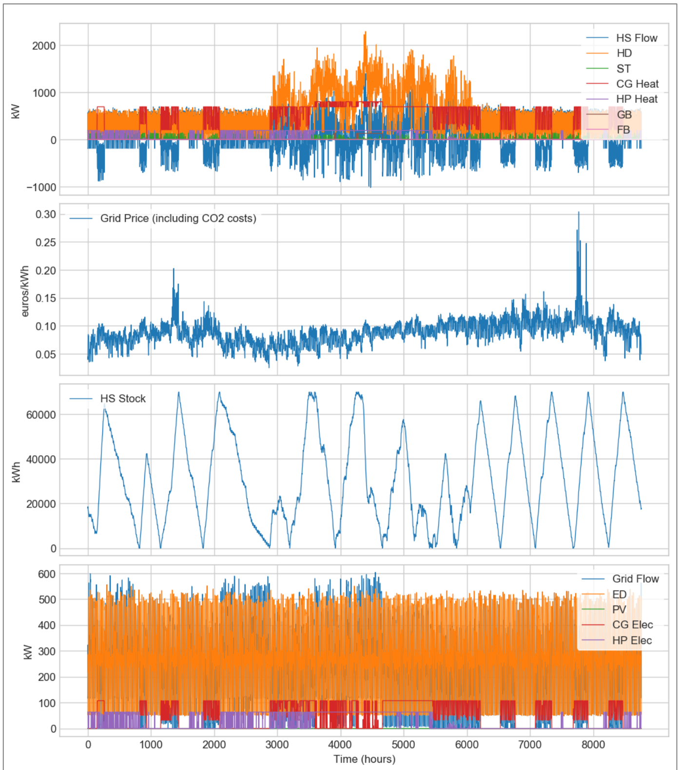
Figure 37: Solution of the OneShot-MILP configuration: heat power balance, grid prices, HS state and electricity balance
