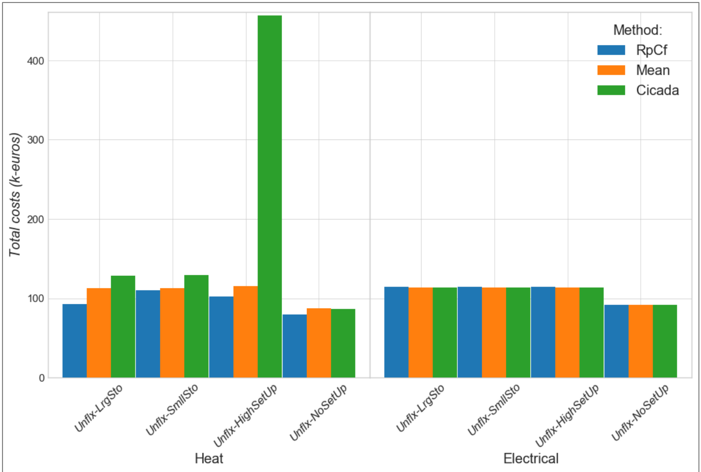
Figure 30: Total costs for the architectures Unflx-LrgSto , Unflx-SmllSto , Unflx-HighSetUp and Unflx-NoSetUp , for Heat and Electrical demand profiles
