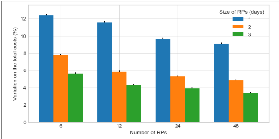
Figure 44: Variation on the total operational costs when method M2 from [23] is used, compared to the reference MILP-OneShot configuration (original problem). This is done for various number and sizes of RPs used within method M2.
