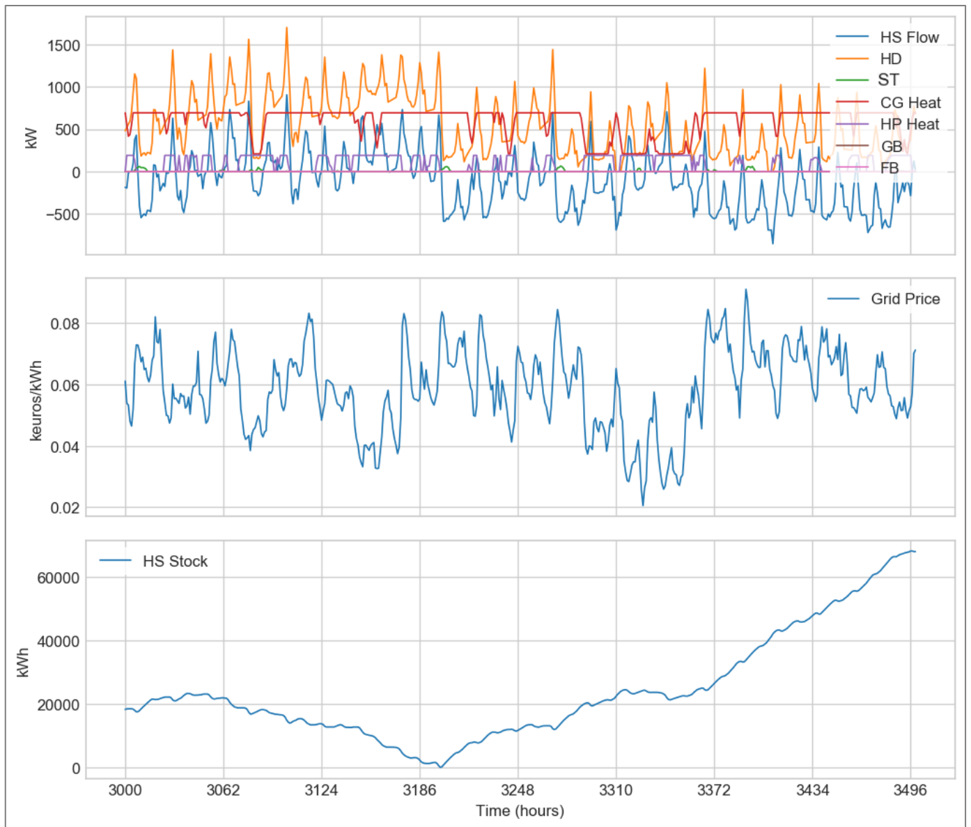
Figure 64: Zoom on the inter-season period, for the MILP-OneShot configuration
