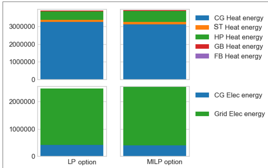
Figure 36: Participation of each source in the HD and ED satisfaction (kWh). Comparison for both LP-OneShot and MILP-OneShot configurations.
