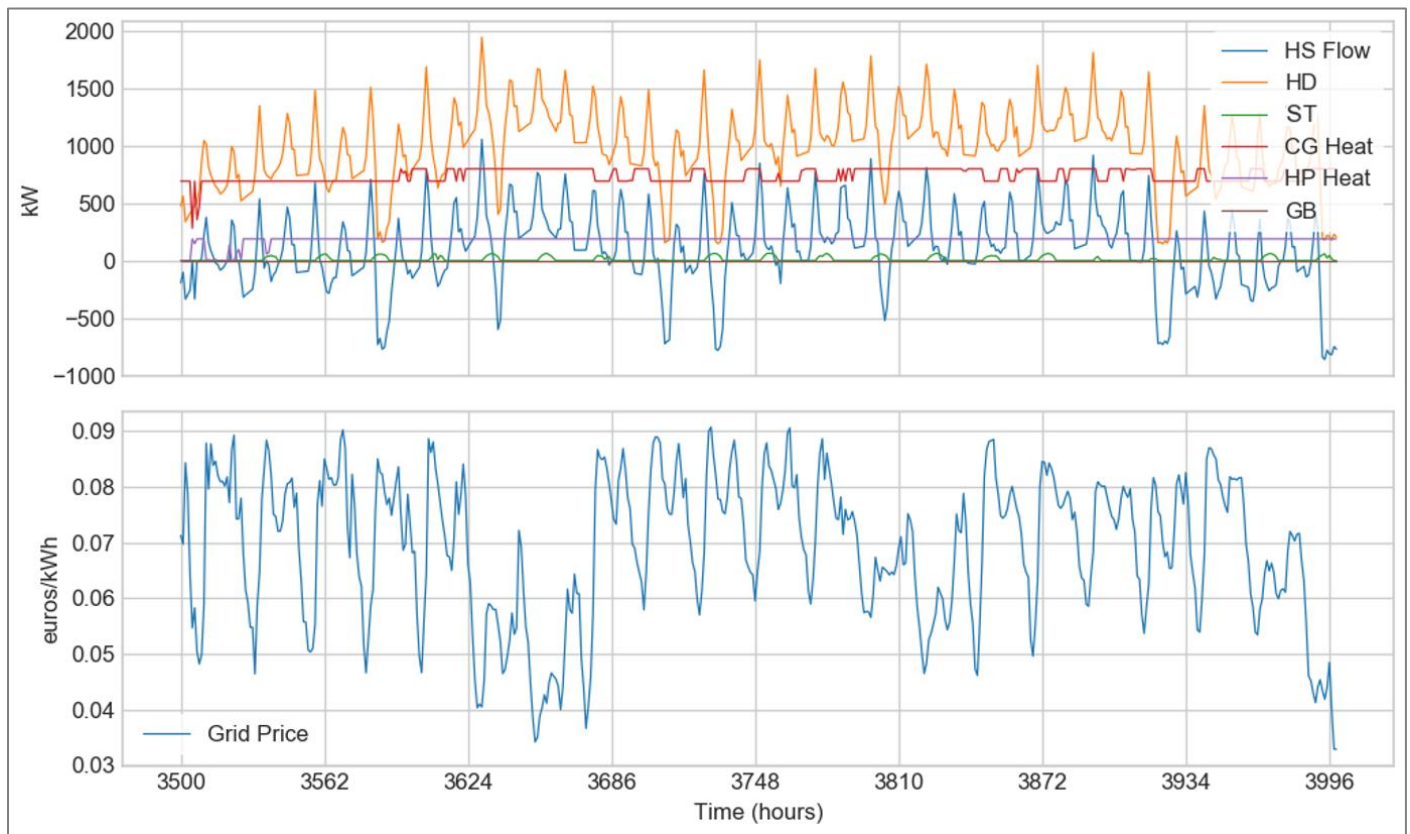
Figure 62: Zoom on the winter period, the strategy is identical for the LP-OneShot and the MILP-OneShot configurations
