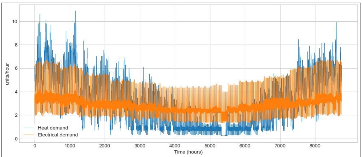
Figure 25: Demand profiles considered (heat and electrical)
