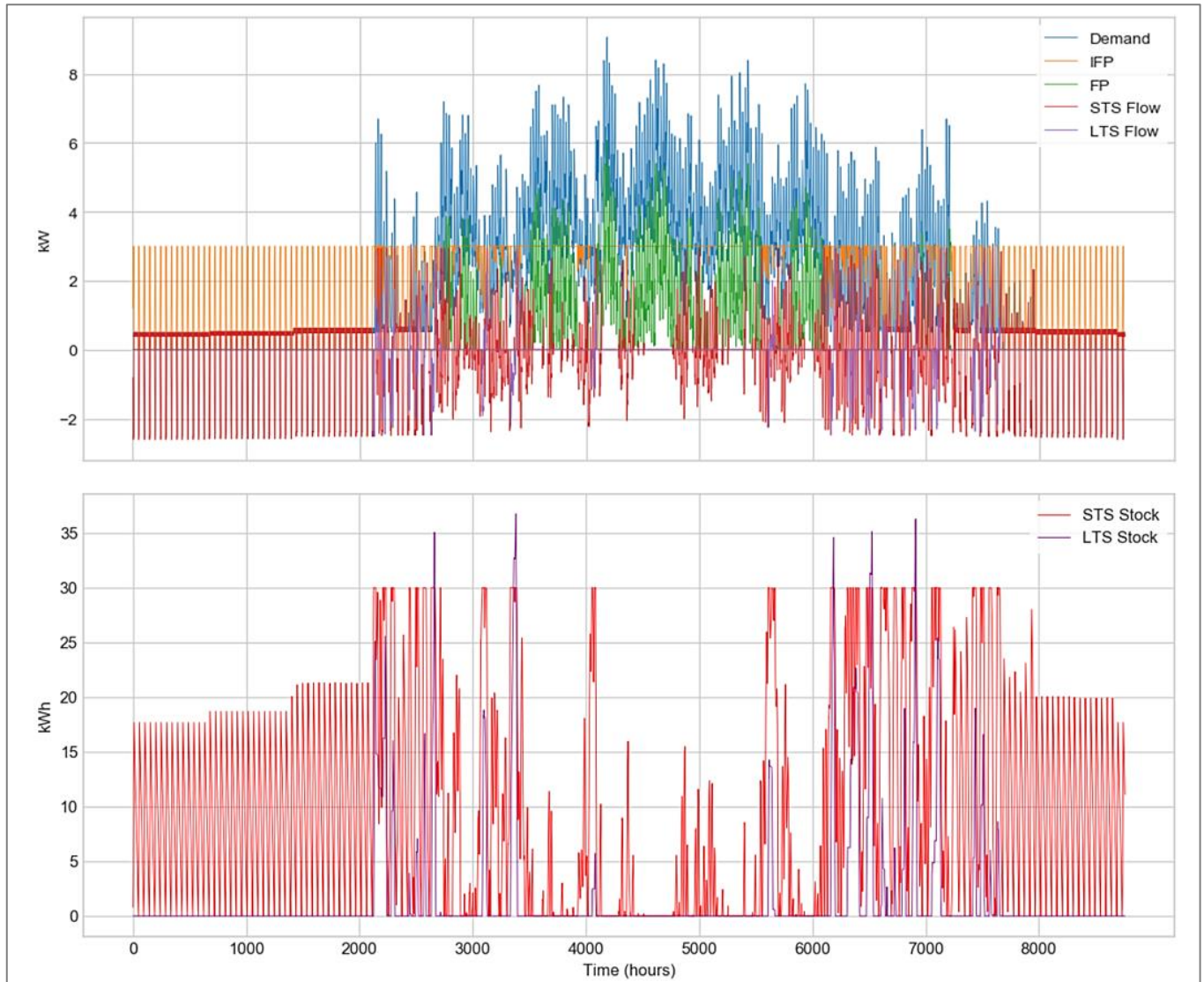
Figure 15: Results for the benchmark Cicada approach.
