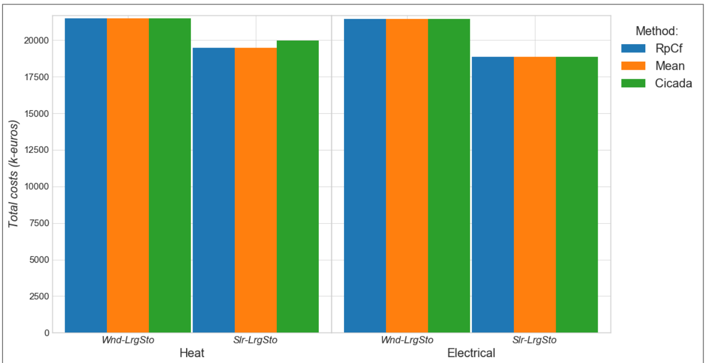
Figure 29: Total costs for the architectures Wnd-LrgSto and Slr-LrgSto, for Heat and Electrical demand profiles
