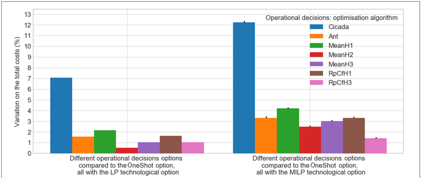
Figure 45: Impact of the operational decisions modelling options.
