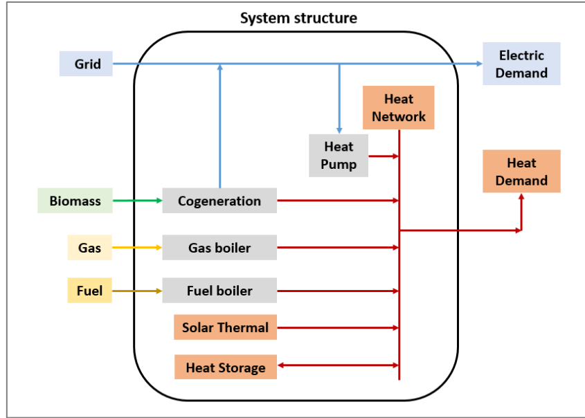
Figure 33: Illustrative case study structure
