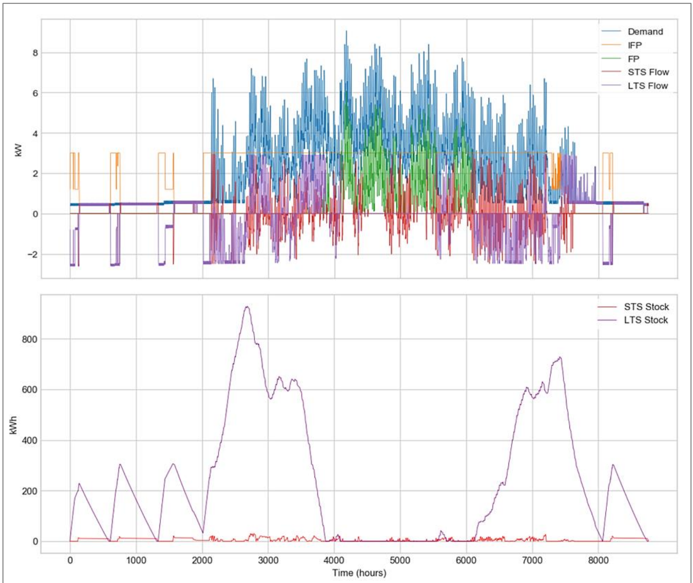
Figure 20: Results for the RpCf-SetUp model, with horizon H1.
