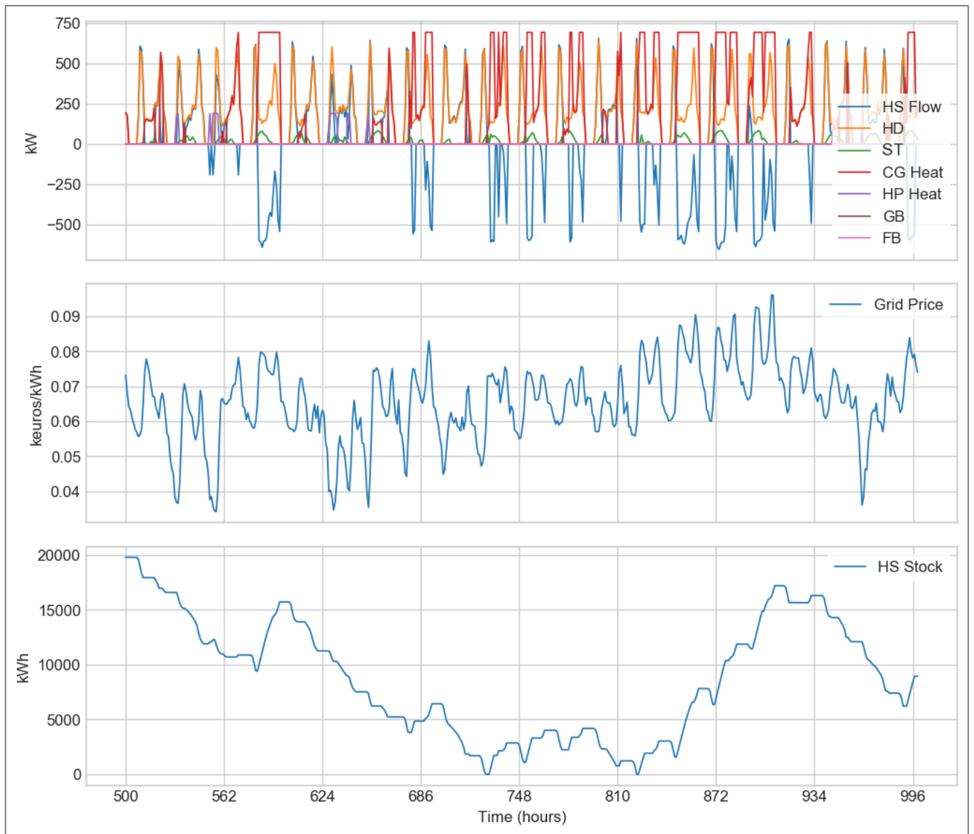
Figure 65: Zoom on the summer period, for the LP-OneShot configuration
