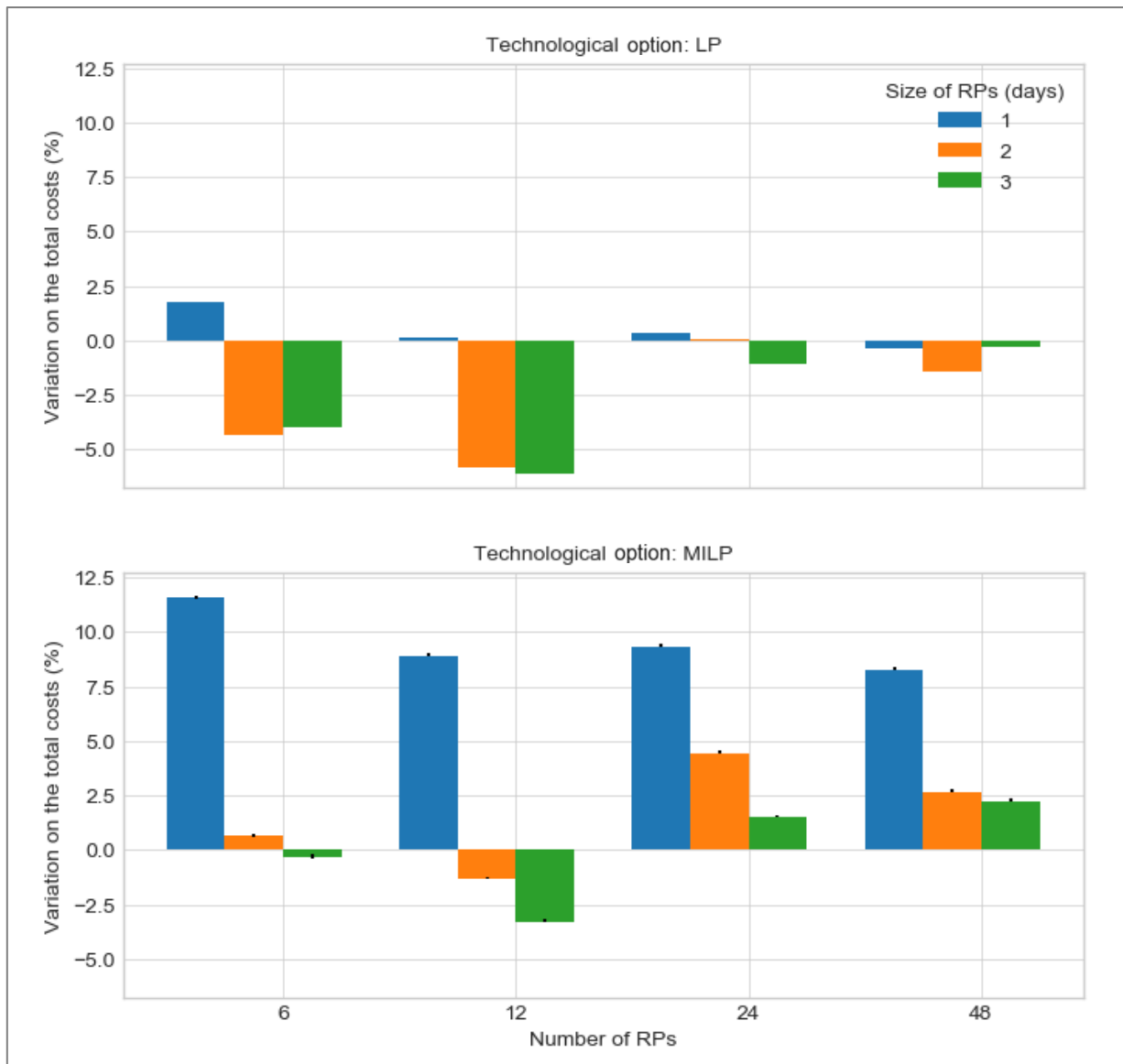
Figure 42: Impact of the temporal aggregation.
