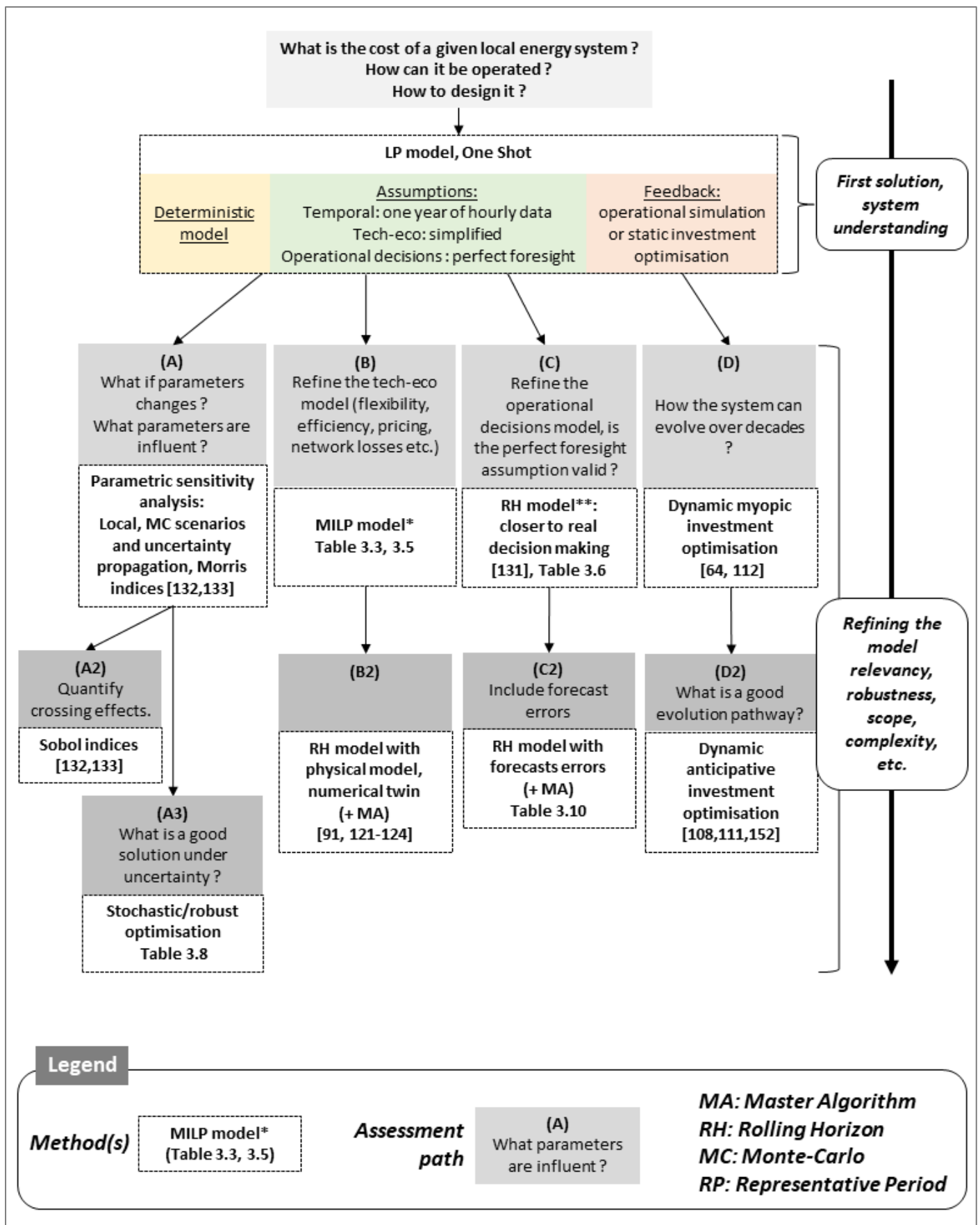
Figure 53: Optional assessment paths when evaluating and optimising an energy system, with possible associated methods *See Figure 54 **See Figure 55
