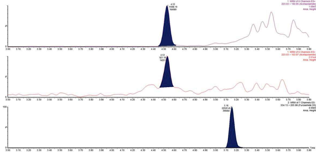
FIGURE 1 Chromatogram obtained after extraction of the 0- to 1-cm hair segment. From top to bottom: Two transitions of acetazolamide and one transition of the internal standard. Drug concentration was 24 \mu\text{g}/\text{mg} [Colour figure can be viewed at wileyonlinelibrary.com ]
