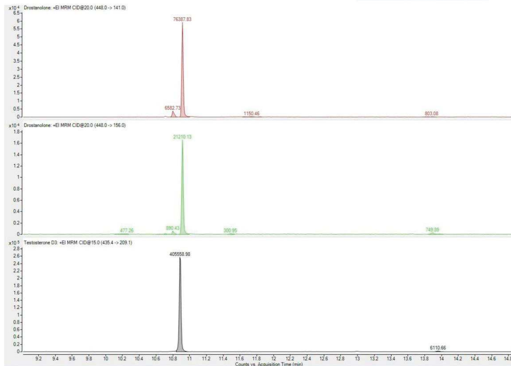
FIGURE 2 Chromatogram obtained after extraction of the fingernail clippings in case 6. Drostanolone concentration was 8 pg/mg. From top to bottom: 2 transitions for drostanolone ( m/z 448.0 > 141.0 and 448.0 > 156.0) and 1 transition for testosterone- d_3 ( m/z 435.4 > 209.1) [Colour figure can be viewed at wileyonlinelibrary.com ]
