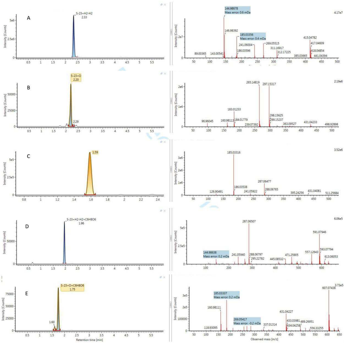
Figure 5: Spectra data information for S-23 and metabolites identified after in vitro incubation, by liquid chromatography coupled to high resolution mass spectrometry (LC-HRMS). (A) S-23 (C 18 H 13 ClF 4 N 2 O 3 ; m/z [M+H] - 415.0478), (B) hydroxyl-S-23 (C 18 H 12 O 4 N 2 ClF 4 ; m/z [M+H] - 431.0423), (C) O-dephenylate-S-23 (C 12 H 10 O 3 N 2 F 3 ; m/z [M+H] - 287.0647), (D) S-23-glucuronide (C 24 H 20 O 9 N 2 ClF 4 ; m/z [M+H] - 591.0794) and (E) hydroxyl-S-23-glucuronide (C 24 H 20 O 10 N 2 ClF 4 ; m/z [M+H] - 607.0743).
