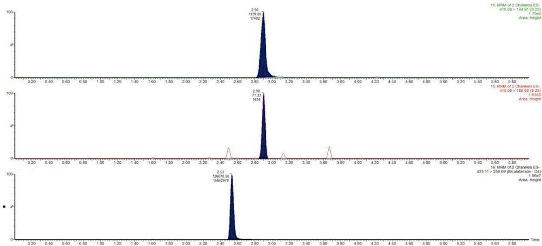
Figure 4: Chromatogram obtained after extraction of urine at + 28 days (672 hours). S-23 concentration was 1 ng/mL. From top to bottom: 2 transitions for S-23 (m/z: 415.1 > 144.9 and 415.1 > 185.0) and 1 transition for bicalutamide-d 4 (m/z: 433.1 > 255.1).
