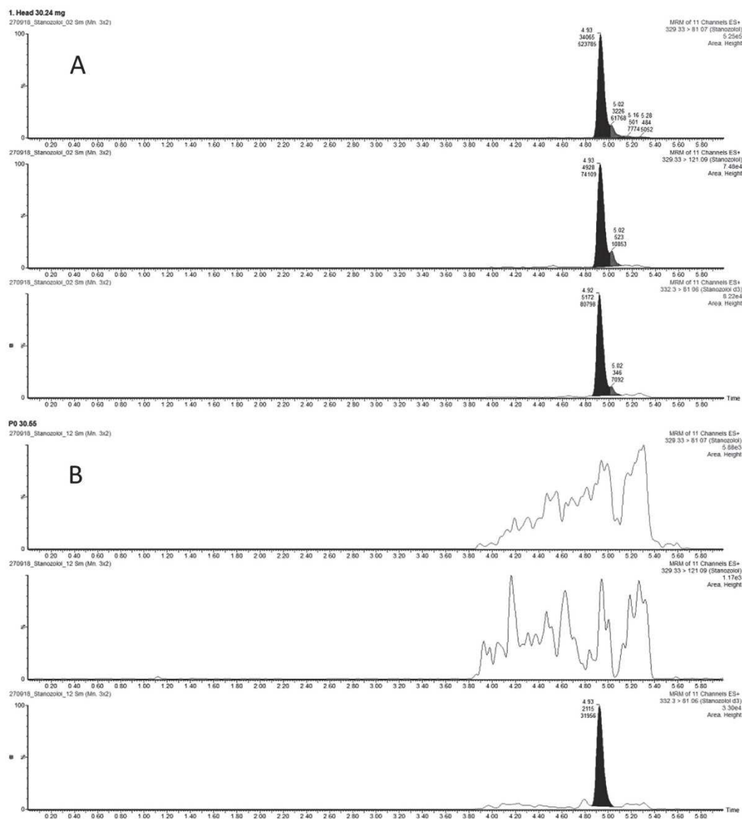
Figure 1. Chromatograms of head hair specimen and blank sample. (A) Head hair; (B) blank hair sample. From top to bottom: first transition of stanzozolol, second transition of stanzozolol, quantification transition of stanzozolol-d 3 .
