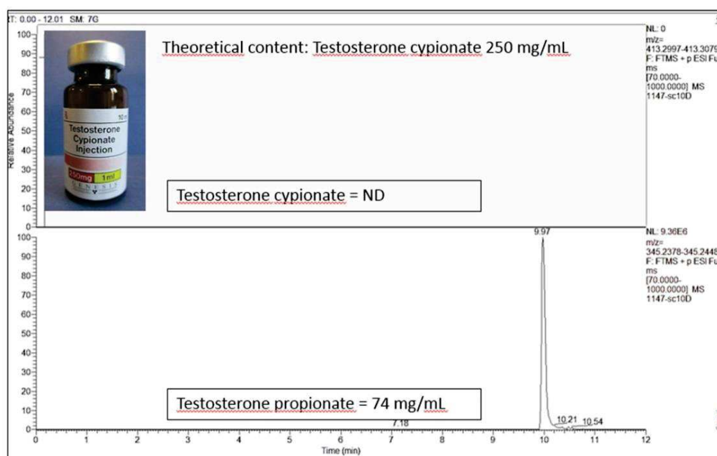
Fig. 1. Photography of sample n°55, theoretical content, experimental content and LC-HRMS extracted ion chromatograms of testosterone cypionate ( m/z=413.3050 ) and testosterone propionate ( m/z=345.2424 ) (ND: not detected).
