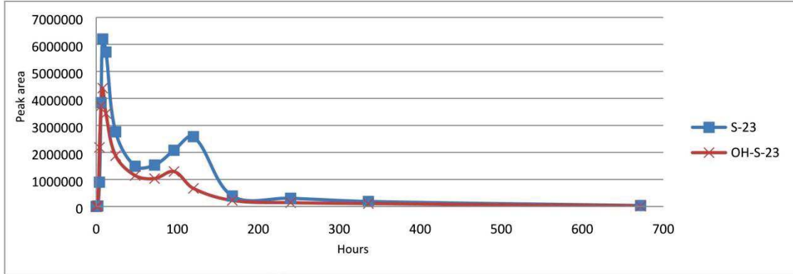
Figure 6: Peak areas of S-23 and hydroxy-S-23
