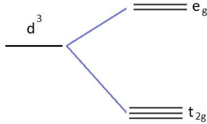
FIGURE 3.2: Electronic structure of an isolated 3d Mn ion degenerance
