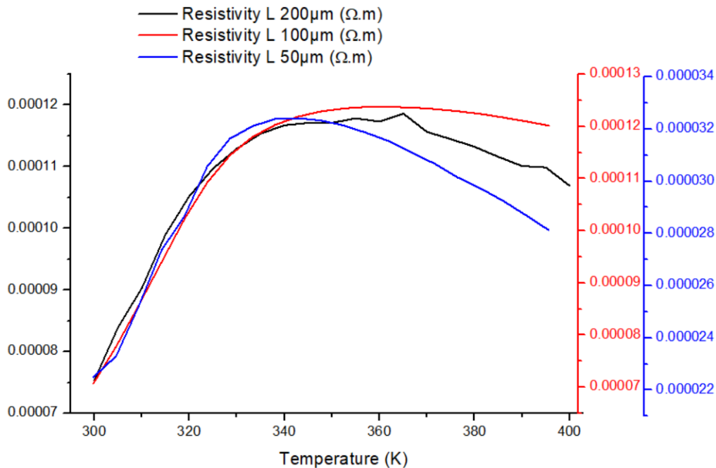
FIGURE 4.34: Suspended 6\ \mu\text{m} large 100\ \mu\text{m} long suspended LSMO resistivity on Si substrate
