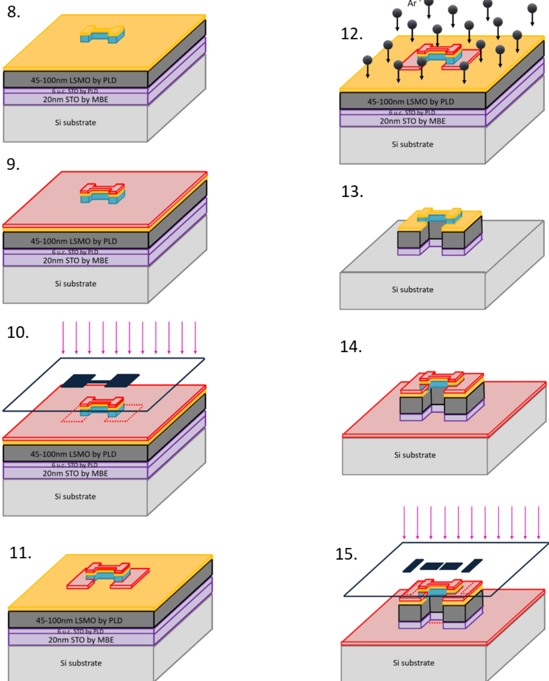
FIGURE 4.36: Schematics of fabrication steps 8-15
