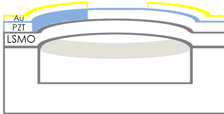
FIGURE 3.8: Piezoelectric actuation on one side of the clamped beam by use of transversal piezoelectric coefficient deformation through drive voltage application between top gold electrode and bottom LSMO thin film.
