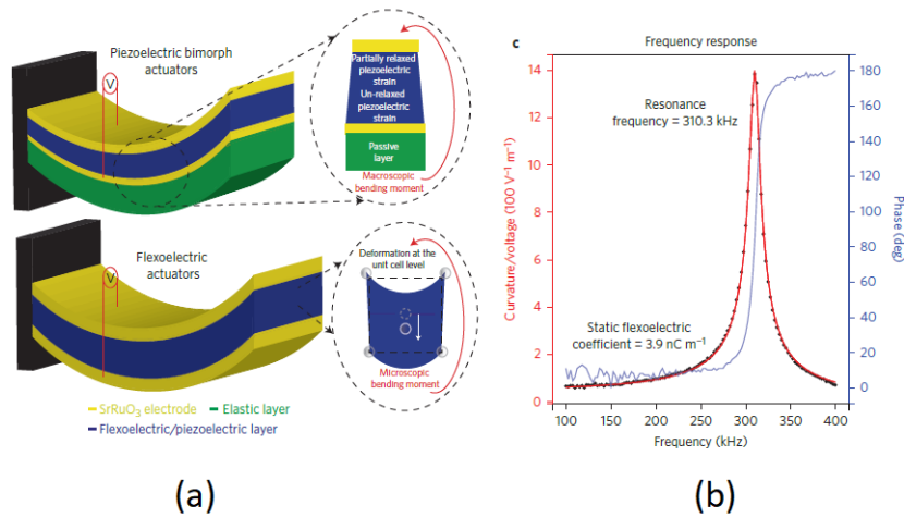
FIGURE 2.15: (a) Schematic comparing flexoelectric actuation and piezoelectric bimorph actuation in nanoscale actuators and (b) curvature/voltage ratio as a function of frequency for the \text{SrTiO}_3 nanocantilever at 1 V excitation, showing the resonant peak at 310 kHz confirmed by the 180^\circ phase change, with quality factor Q of 25. Extracted from (Bhaskar et al., 2016)
