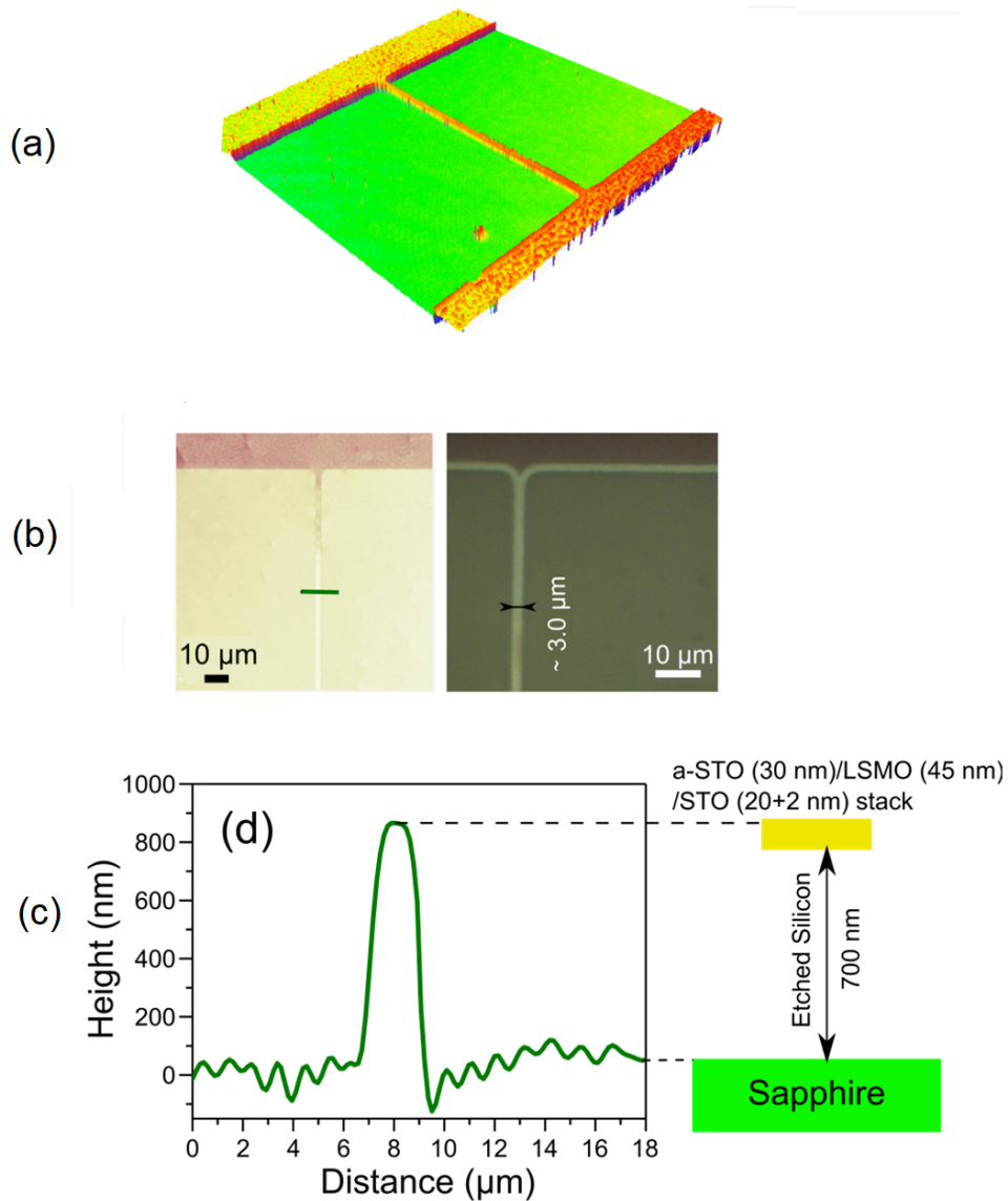
FIGURE 4.31: (a) 3D-reconstruction image in DHM R2200, (b) phase numerical reconstructions image in DHM with topographic information on the sample and optical microscope image of a 3\ \mu\text{m} wide 100\ \mu\text{m} long suspended bridge and the (c) thickness profile at the center position obtained from phase information
