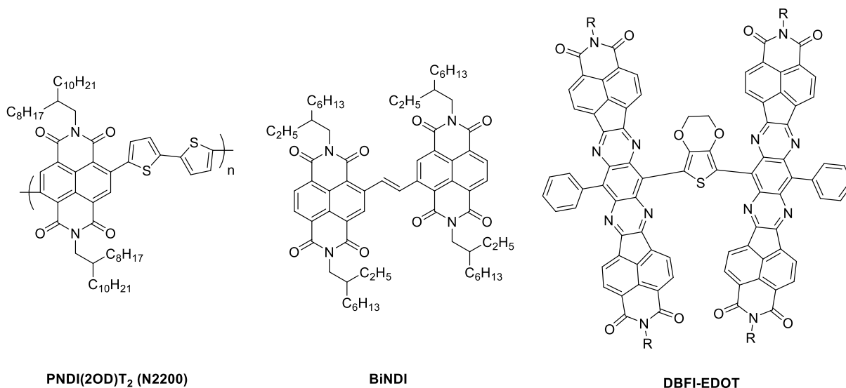
Figure 18. Chemical structure of naphthalene mono- and diimide derivatives for NFA-based OSCs.
