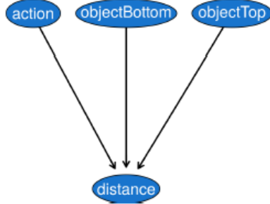
Figure 3.8: Conditional linear Gaussian network obtained after learning process.
