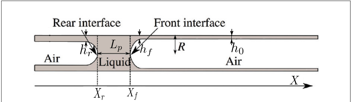
Figure 2.1 – Sketch of a liquid plug in a prewetted capillary tube adapted from [97].
