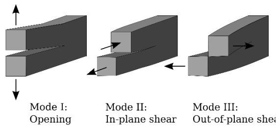
Figure 48. Fracture modes allowing cracks propagation in materials
