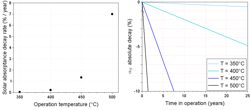
Figure 60. Solar absorptance yearly decay rate vs. operation temperature (left) and solar absorptance absolute decay vs. time in operation (right) of a TiAlN coating at PROMES [253]
