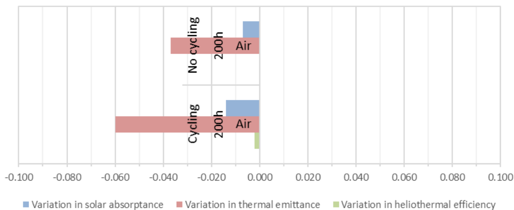
Figure 131. Variation of the optical properties for cycling and non-cycling aging treatments for the WAISiN absorber
