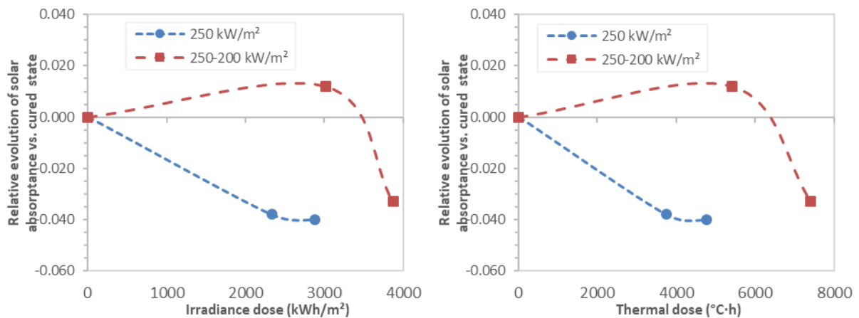
Figure 160. Relative evolutions of solar absorptance with constant ( 250 \text{ kW}^2 ) and cyclic ( 250\text{-}200 \text{ kW/m}^2 ) solar aging vs. cured state (0h), vs. irradiance dose (left) and thermal dose (right) received by the samples
