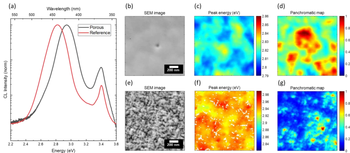
Figure 4-9. (a) Normalized integrated CL spectra in logarithmic scale of the middle region for the porous sample, in black, and reference sample, in red. SEM picture of the analysed region in (e) and (b) respectively. (c) and (f) are the peak energy position maps for the reference and porous sample, respectively. Panels (d) and (g) are the respective panchromatic maps.
