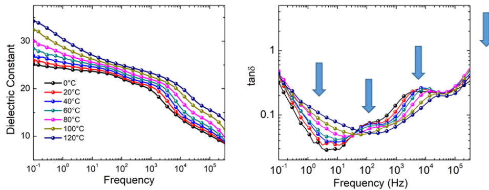
Figure 60 Dielectric constant and \tan \delta of Al 2 O 3 /ZnO (0.2/0.5 nm) laminate as a function of frequency and temperature
