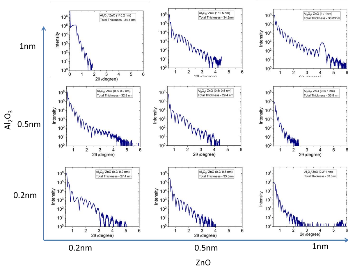
Figure 55 XRR spectra of \text{Al}_2\text{O}_3/\text{ZnO} laminates deposited at 0.005mbar oxygen pressure.
