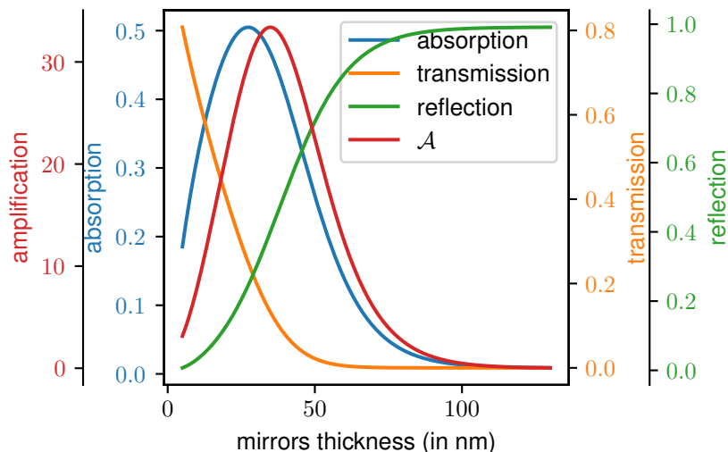
Figure 3.14: Intracavity amplification factor \mathcal{A} , total absorption, transmission and reflection against thickness. Computations are made with a constant refractive index corresponding to a 50 nm layer of silver. Note that the points where the curves cross are not significant because each curve has its own scale.
