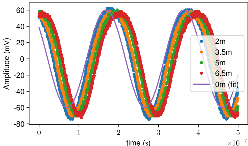
Figure D.1: Signal from the PhotoDiode (PD) with different cable length. This permits to extract the phase relation to cable length, hence to extrapolate the actual signal with a 0 m long cable.
