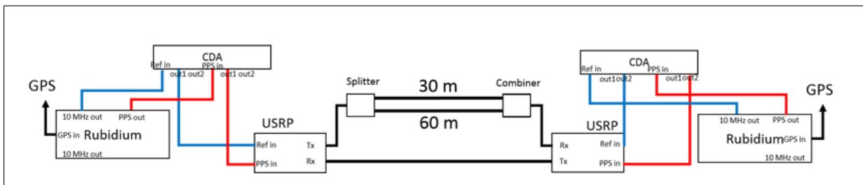
Figure 4.16: Propagation test with cables of 60 meters
