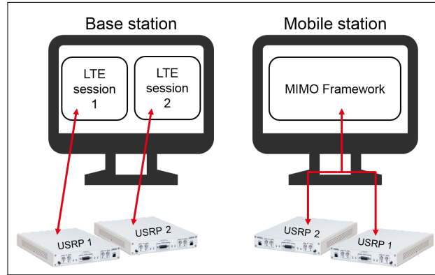
Figure 4.6: Software architecture
