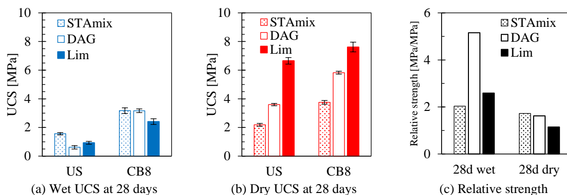
Figure 3.29. Wet (a) and Dry (b) UCS of STAmix, DAG and Lim – unstabilized (US) and stabilized with 8% of CB (CB8)
