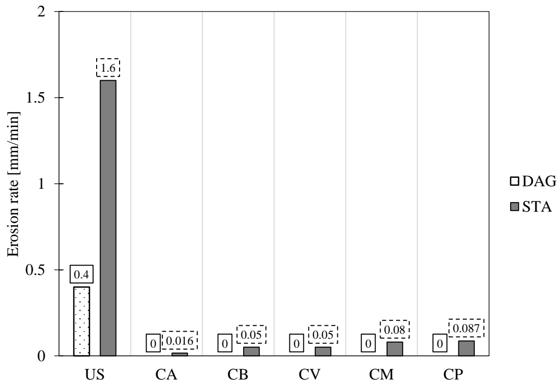
Figure 3.17. Erosion rate of DAG and STA formulations
