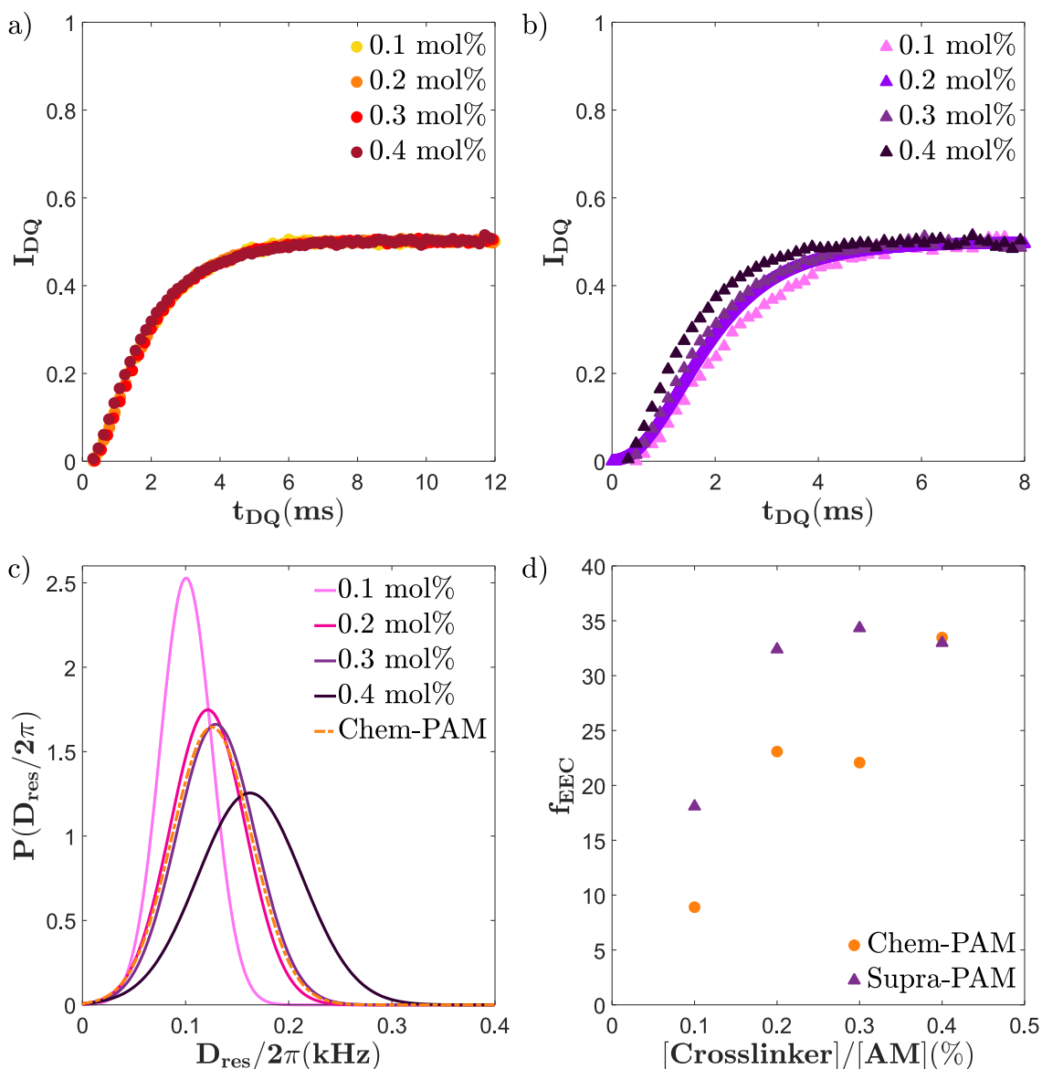
Figure 8. Normalized DQ intensity, I_{DQ} , as a function of ^1H DQ excitement time, t_{DQ} , for (a) Chem-PAM and (b) Supra-PAM gels. (c) Distribution of D_{res} , P(\frac{D_{res}}{2\pi}) , deduced from the fit of the data reported in (a) and (b) using a Gaussian distribution. (d) Evolution of the fraction of the repeat units involved in elastically effective polymer chains, f_{EEC} , with crosslinker feed ratio for Chem-PAM and Supra-PAM hydrogels.
