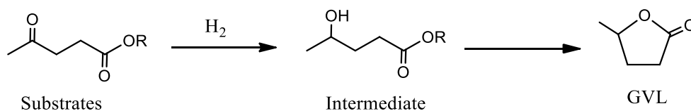
Figure 1.16. Possible mechanism of hydrogenation of LA and its esters with H 2 to GVL.
