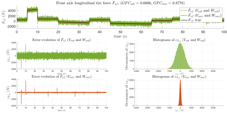
Figure 5.31: F_{xf} estimates. The upper plot shows the true signal (in black) and its estimates with W_{sub} , V_{sub} (in green) and W_{mix} , V_{mix} (in red). The bottom left figures illustrate the evolution of the residuals. The bottom right plots display the error histograms.
