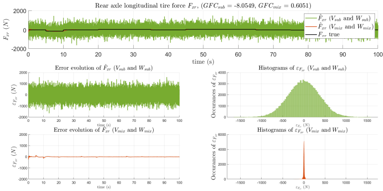
Figure 5.32: F_{xr} estimates. The upper plot shows the true signal (in black) and its estimates with W_{sub} , V_{sub} (in green) and W_{mix} , V_{mix} (in red). The bottom left figures illustrate the evolution of the residuals. The bottom right plots display the error histograms.
