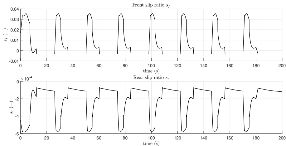
Figure 5.45: Front and rear slip ratios VI-CRT simulated data.
