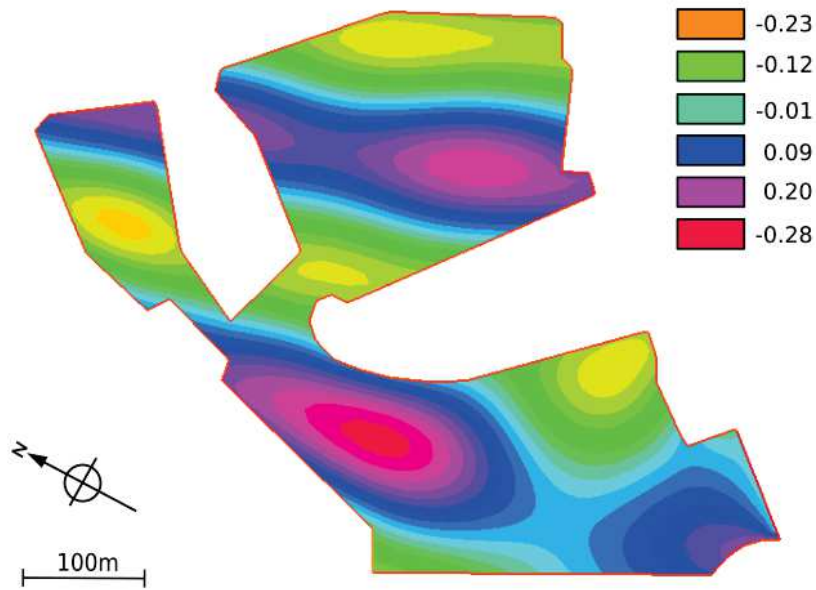
Figure 1.26: Example of reflected wave field, resulting from the resolution of the Helmholtz equation, with (\theta, f, a_{\max}) = (245, 0.0186, 0.172)
