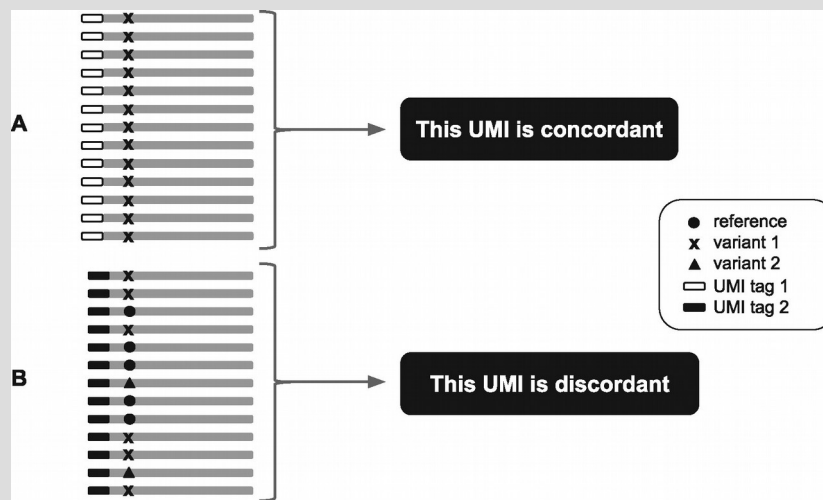
Figure 56: Classification des UMI concordants et discordants.
