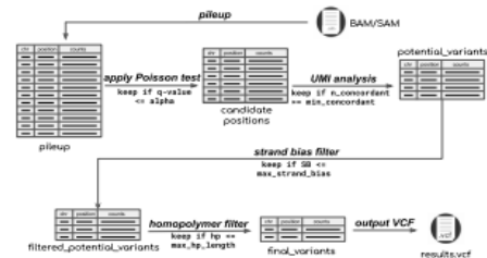
Fig. 3. UMI-VarCal workflow: UMI-VarCal starts by building a pileup from the BAM/SAM file provided. The pileup consists on A,C,G,T, insertion and deletion counts for each position covered by the alignment file. Since we know that not all positions contains mutations, UMI-VarCal starts looping through the pileup and applying a Poisson test at each position to filter out positions that don't seem to contain variants. To each of these candidate positions, an UMI analysis is carried out. At this step, one of 2 conditions are required in order to keep the variant. If the UMI analysis is successful, the potential variant must go through a strand bias filter to make sure that it isn't strand biased. If it passes that test, a final homopolymer region length filter is applied to make sure that the alternative allele is not due to the variant's presence in a long homopolymer region. If the alternative allele passes all these filters, it will be called and present in the final VCF file.
