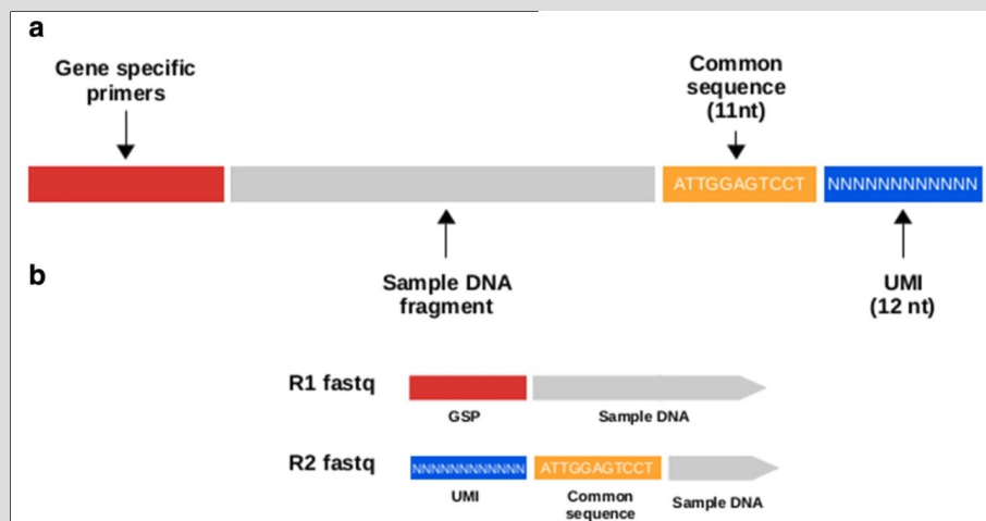
Figure 47: Construction des librairies QIAseq.
