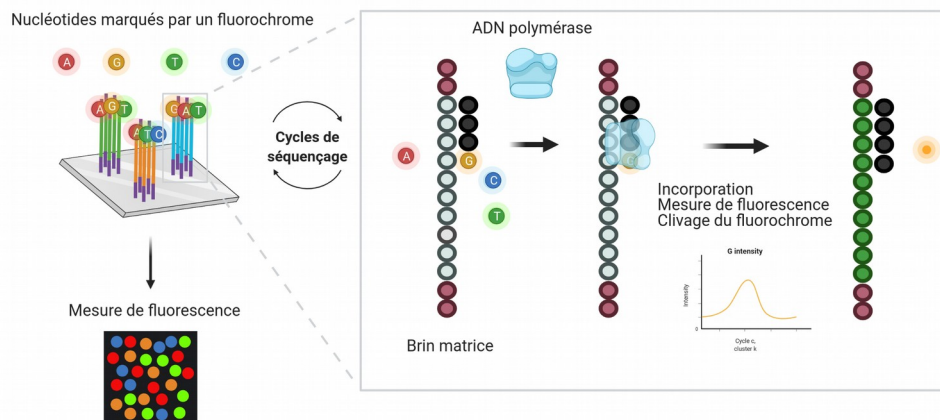
Figure 25: Séquençage Illumina
