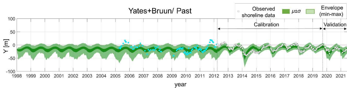
Figure D.5. Ensemble shoreline evolution simulated using the combined Yates and Bruun models, including the envelope (light-shaded areas) and the standard deviation intervals ( \mu \pm \sigma ) (dark-shaded areas) of the 10000 simulated shoreline trajectories, respectively, over the 1998-2021 period (‘past scenario’). Black dashed lines delimit the calibration and validation periods, including shoreline observations (white circles). Cyan circles indicate shoreline data prior to March 2012.
