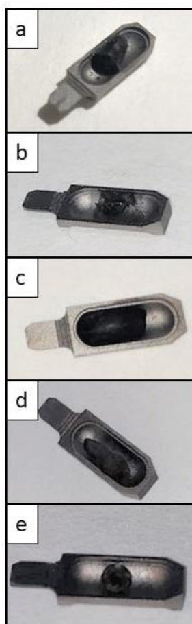
Figure 6. Devices after GFAAS temperature programme (See Table 1 ). a) Mitra using Pd; b) Mitra using Pt; c) HemaXis DB10 using Pt; d) Capitainer qDBS using Pt and e) HemaPEN using Pt.
