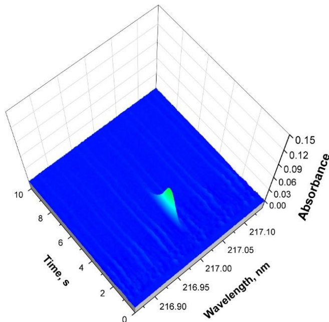
Figure 7. Time- and wavelength-resolved spectrum from Figure 1A (vicinity of 217.000 nm, spectral window 0.28 nm) corrected using TAP correction model.
