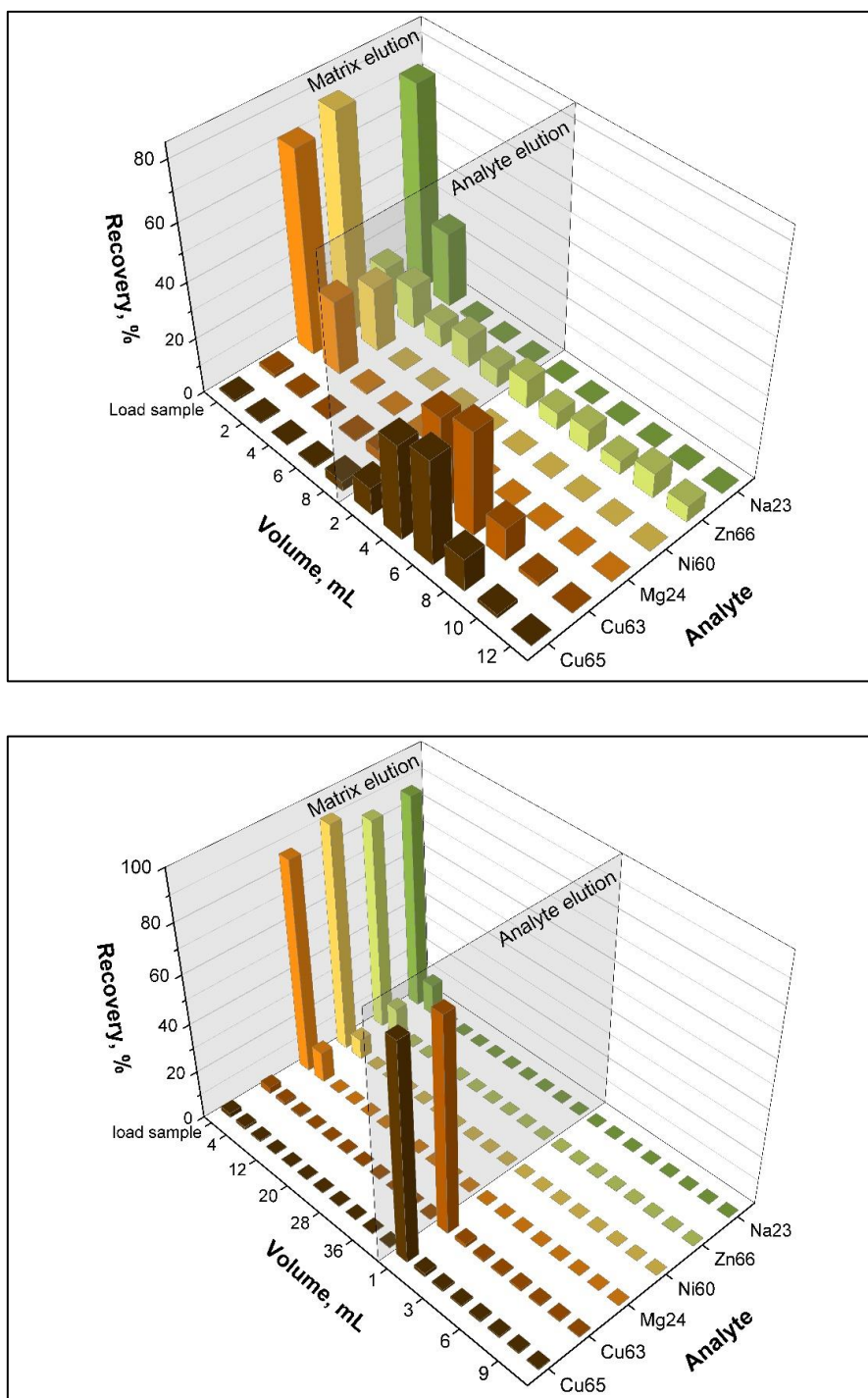
Figure S3. A) Elution profile for selected elements using AG-MP1 resin (Bio-Rad). B) Elution profile for selected elements using Cu-specific resin (Triskem). The Clincheck whole blood reference material L-3 (as described in section 2.3) was measured.
