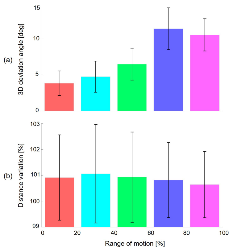
Fig. 5.12 (a) 3D deviation angle between both knee and the orthosis mean AoR as a function of the knee RoM for all eight subjects. (b) Mean distance variation from the wearer HJC to the robotic knee joint center as a function of the knee RoM.
