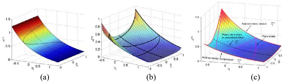
Figure 2.6: Different fracture locus: (a) Johnson-Cook model independent of Lode angle; (b) Symmetric fracture locus with Lode angle dependency proposed by Xue and Wierzbicki[Xue08];(c)Asymmetric fracture locus with Lode angle dependency proposed by Bai and Wierzbicki [Bai08].
