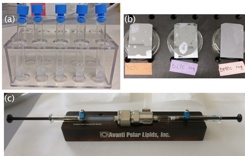
Figure 13: (a) Example of sample appearance after extrusion through a 100 nm membrane. The ones shown are five copies of C10 mix 80 mM in bicine 0.2M at T = 25^{\circ}\text{C} . (b) Example of flat multilayers prepared by spreading organic solutions on silicon flat wafers, before annealing. From left to right: DCPC (C10), DLPC (C12), DMPC (C14). (c) Equipment used for the extrusion, provided from Avanti Polar Lipids (Alabaster, AL).
