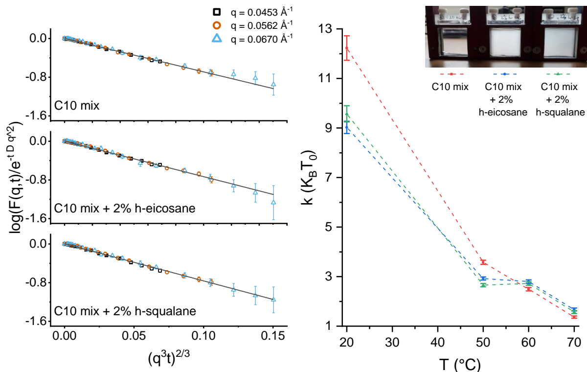
Figure 5. Left: NSE data at T = 70^\circ\text{C} plotted in the representation \log[F(q, t)/\exp(-Dq^2t)] vs (q^3t)^{2/3} . This highlights the stretched exponential decay predicted by the Zilman-Granek theory [41] and additionally shows that a more complex model taking into account the lipid droplet signal is unnecessary (details in the “Materials and Methods” section). Right: plot of the bending rigidity estimates as a function of the temperature. Inset shows the sample appearance after the NSE thermal scans.
