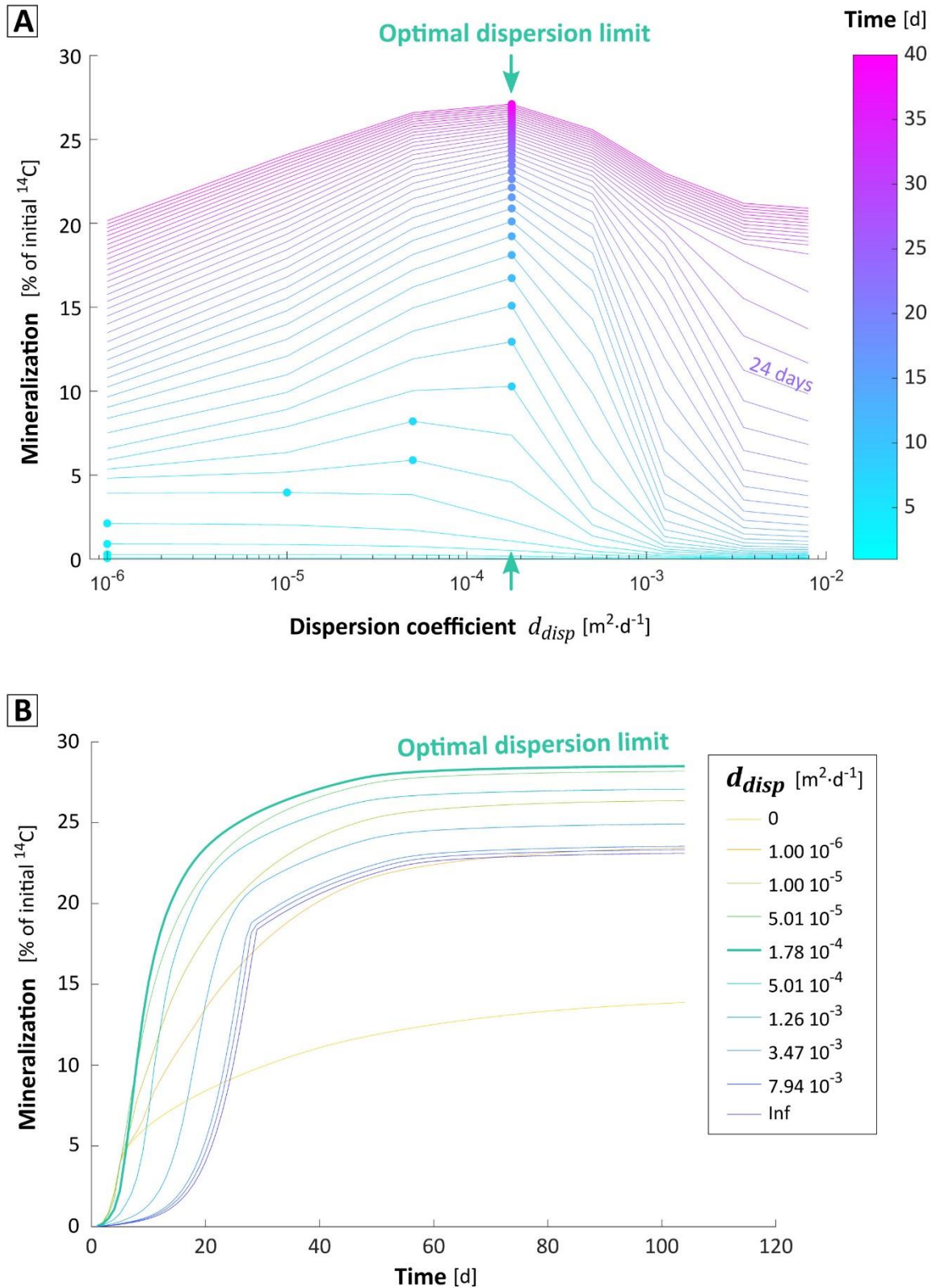
Fig. S9. Convergence of optimal bacterial spreading with time. (A) Daily mineralization values depending on bacteria dispersion coefficients d_{disp} , for the parameter set calibrated under Monod model on both hydrostatic and percolation experiments. For each day represented by the color scale, the optimal dispersion is indicated with a dot. (B) Dynamics of mineralization for each d_{disp} .
