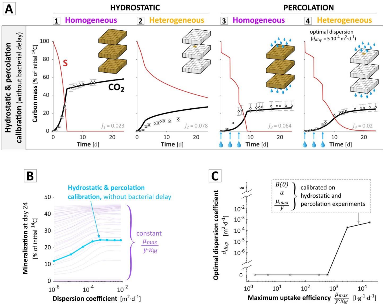
Fig. S6. Main modeling results without the explicit bacterial accommodation rate \alpha based on Patarinska et al. (2000). This accommodation function induces a permanent delay in the observed specific growth rate \mu , which tends towards its value derived from the Monod relation, following a concave relation whose half-life is given by \alpha . For representation and legend, see Fig. 3, 4 and 6.
