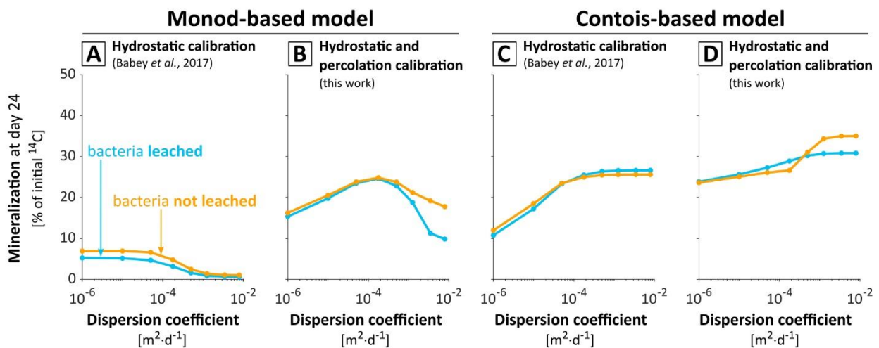
Fig. S4. Impact of dispersion on mineralization predicted at day 24, depending on the scenario of bacteria leaching. During the percolation events, bacteria were either leached at the same rate as the substrate (blue lines) or not leached (orange lines). The panels represent the relation between the dispersion coefficient d_{disp} and the final mineralization for the hydrostatic Monod calibration (Babey et al., 2017) applied to the Monod-based (A) and the Contois-based (C) models, and for the two parameterizations calibrated in this work on both hydrostatic and percolation experiments under Monod-based (B) and Contois-based (D) models. The parameterizations calibrated under the Monod-based and the Contois-based models are described respectively in sections 3.1 and 3.3, and parameter values are given in table 2 . As illustrated here, bacteria leaching did not affect the existence of an optimal dispersion for bacteria and its dependence on the maximum uptake efficiency.
