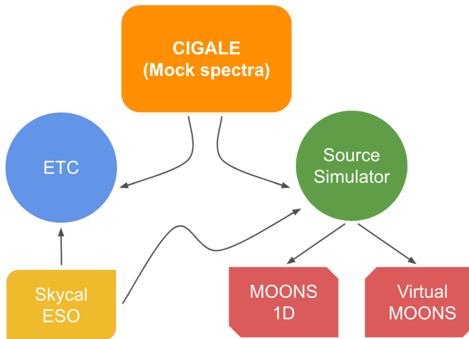
Figure 6.2. – Simulation tools flow chart. The mock spectra created with CIGALE in our case or with any other tool are passed directly to the ETC and the source simulator. Both contain the ESO sky model (Noll et al., 2012). Once the sources are treated by the Source Simulator, they can be used in the MOONS 1D spectra simulator or in Virtual MOONS to obtain final reduced science mock spectra. The figure is inspired by a figure presented by Myriam Rodrigues at the MOONS consortium science meeting.
