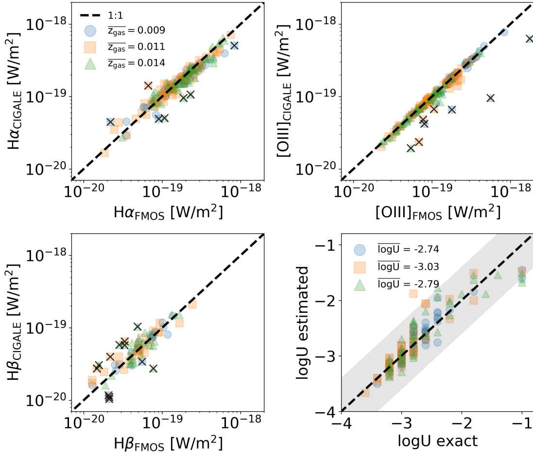
Figure 4.3. – Quality of the fits including H\alpha , H\beta , and [OIII]\lambda 5007 emission lines, and ionization parameter estimation. From left to right, top to bottom, we show the CIGALE fit versus observed flux for the H\alpha , [OIII]\lambda 5007 , H\beta emission lines. The three different gas-phase metallicity bins are presented as blue circles, orange squares, and green triangles. The black crosses correspond to excluded data with flux differences larger than 0.2 dex. The black line corresponds to the 1:1 relation. The three emission lines are well fitted for the three different median gas-phase metallicity models. The last panel shows the estimated versus exact value for \log U from mock samples created with CIGALE. Symbols are the same as the legend in the first panel and the median ionization parameter value is shown. The shaded area corresponds to the standard deviation.
