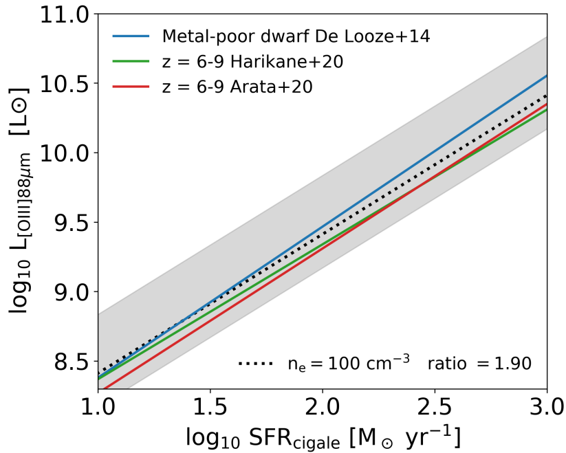
Figure 3.17. – [OIII] 88 \mu\text{m} -SFR relation. The blue line shows the metal-poor local dwarf galaxies relation from De Looze et al. (2014). The green line corresponds to the high-redshift observed relation proposed by Harikane et al. (2020) while the red line corresponds to simulation results from Arata et al. (2020) both at z = 6 - 9 . We translate our [OIII] \lambda 5007 luminosities into [OIII] 88 \mu\text{m} using a mean ratio of 1.9 derived from CLOUDY HII-region models at an electron density of n_e = 100 \text{ cm}^{-3} shown as a black dotted line. The gray area is the dispersion in the translation with gas-phase metallicity.
