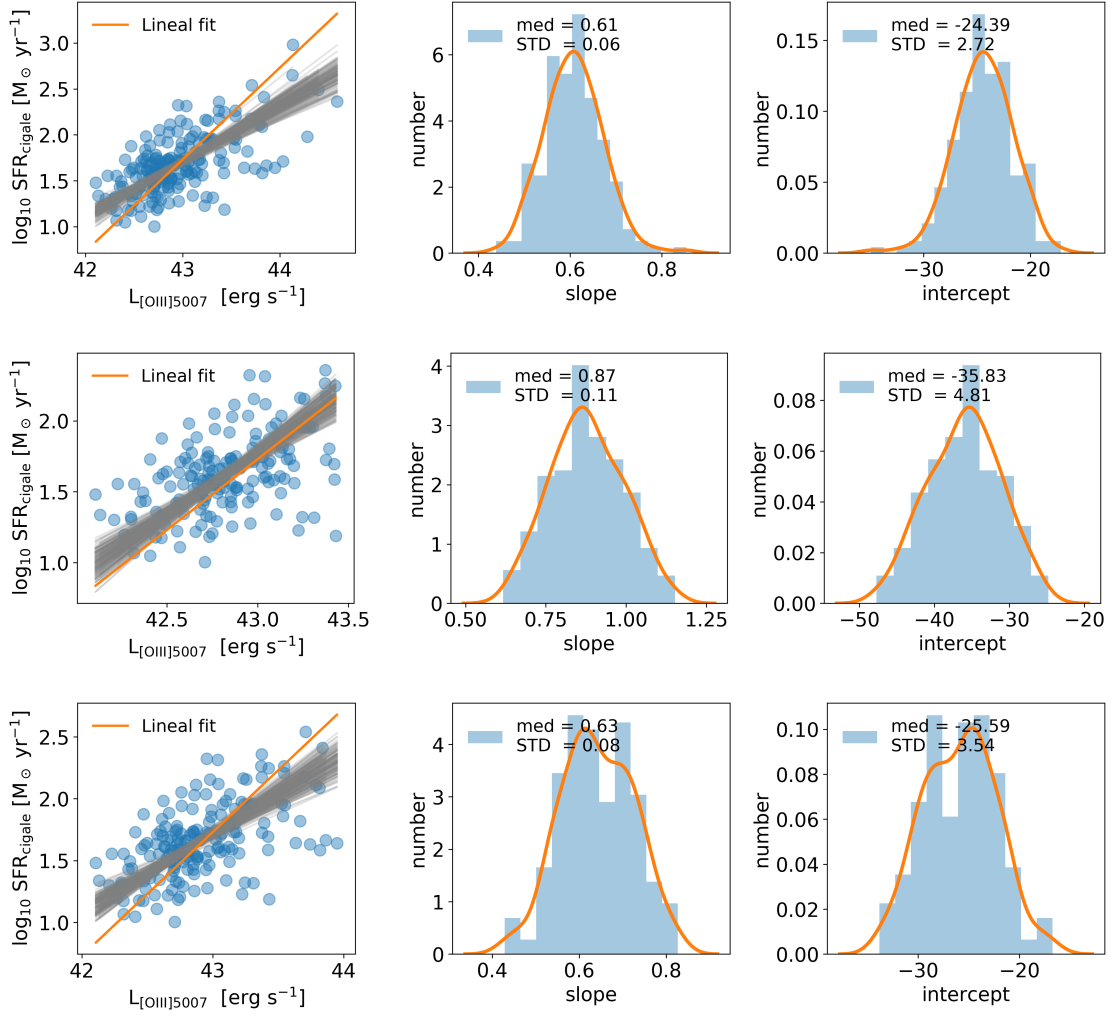
Figure 3.15. – Orthogonal distance fitting with both slope and intercept varying. top: Entire sample; center: L_{[\text{OIII}]\lambda 5007} \leq 10^{43.5} \text{ erg s}^{-1} ; bottom: L_{[\text{OIII}]\lambda 5007} \leq 10^{44} \text{ erg s}^{-1} . The orange line represents the linear fit from Eq. 3.6 while the gray lines correspond to 200 realizations of the bootstrapping process. The estimated distribution after bootstrapping of the slope and intercept are presented in the middle column and the right column, respectively. Slope estimates vary strongly on the way luminosities are clipped as this changes the distribution of L_{[\text{OIII}]\lambda 5007} and SFR.
