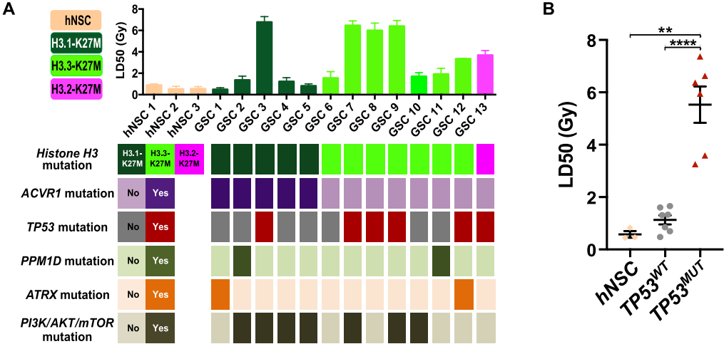
Figure 2. Correlation of the mutational landscape of DIPG cellular models to in vitro radiosensitivity. A , Average LD50 were determined in vitro in 3 NSCs and 13 DIPG GSCs from at least 3 independent assays (top). Genomic alterations detected in histone H3 ( H3F3A , HIST1H3B/C , HIST2H3A/C ), ACVR1 , TP53 , PPM1D , ATRX as well as components of the PI3K/AKT/mTOR pathway in the corresponding GSCs are indicated (bottom). B , Measured LD50 (Gy) were stratified according to human neural stem cells (hNSC), TP53 WT GSCs and TP53 MUT GSCs (Student's t-test, **, p = 0.0015 ; ****, p < 0.0001 ). Results are expressed as mean ± SD.
