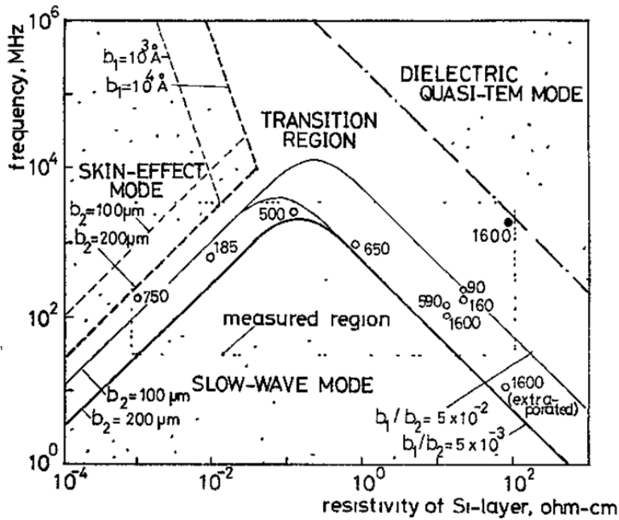
Figure 119 : Resistivity-Frequency domain chart. Permittivity of SiO 2 and Si, 4 and 12 respectively. The hollow points and full points are measured Slow-wave and TEM modes respectively. Numbers next to them give the width of the microstrip.[294]
