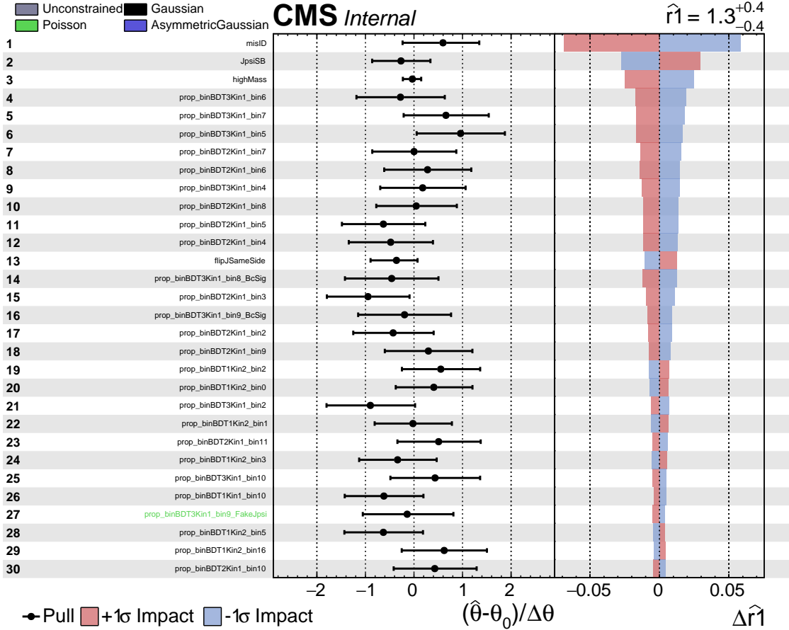
FIGURE 6.10: Impacts of the nuisance parameters on r_1 (signal normalisation in the first p_T^{\text{HMM}} bin), in the pp second-step fit.
