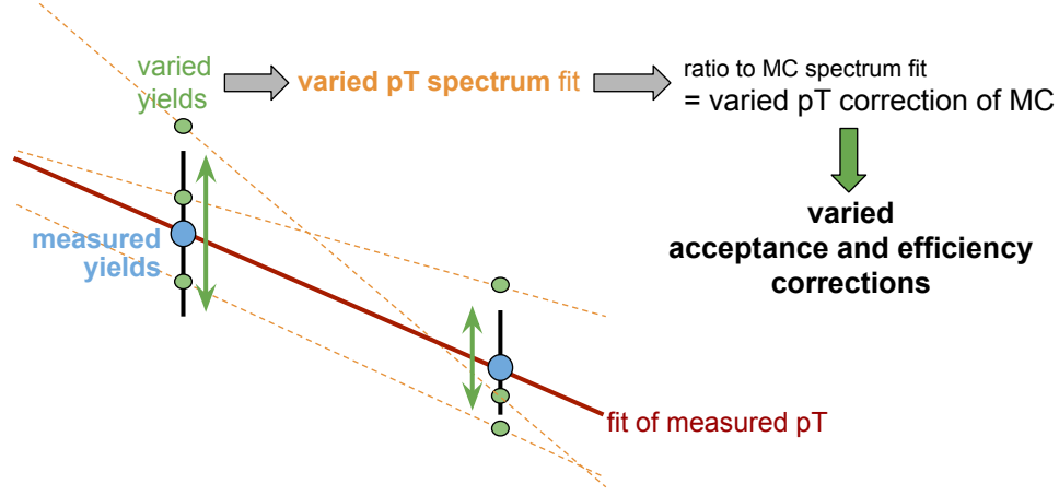
FIGURE 7.33: Extraction of the uncertainties on the acceptance and efficiency corrections from variations of the measured p_T^{\text{muon}} spectrum.
