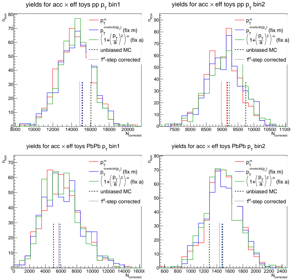
FIGURE 7.37: Variations of the second-step data measurement are associated to variations of the p_T^{\text{MUU}} spectrum correction in MC. Here is shown in the two p_T^{\text{MUU}} bins in pp (top) and PbPb (bottom) the effect of these variations on the corrected yields, including the uncertainty on the measurement of the observed yields. The coloured dashed lines are the nominal results from the three p_T^{\text{MUU}} -spectrum fit functions (and no variation of the data points), compared to the original result without any correction of the p_T^{\text{MUU}} spectrum (dashed black line) or with the first-step correction (dotted line).
