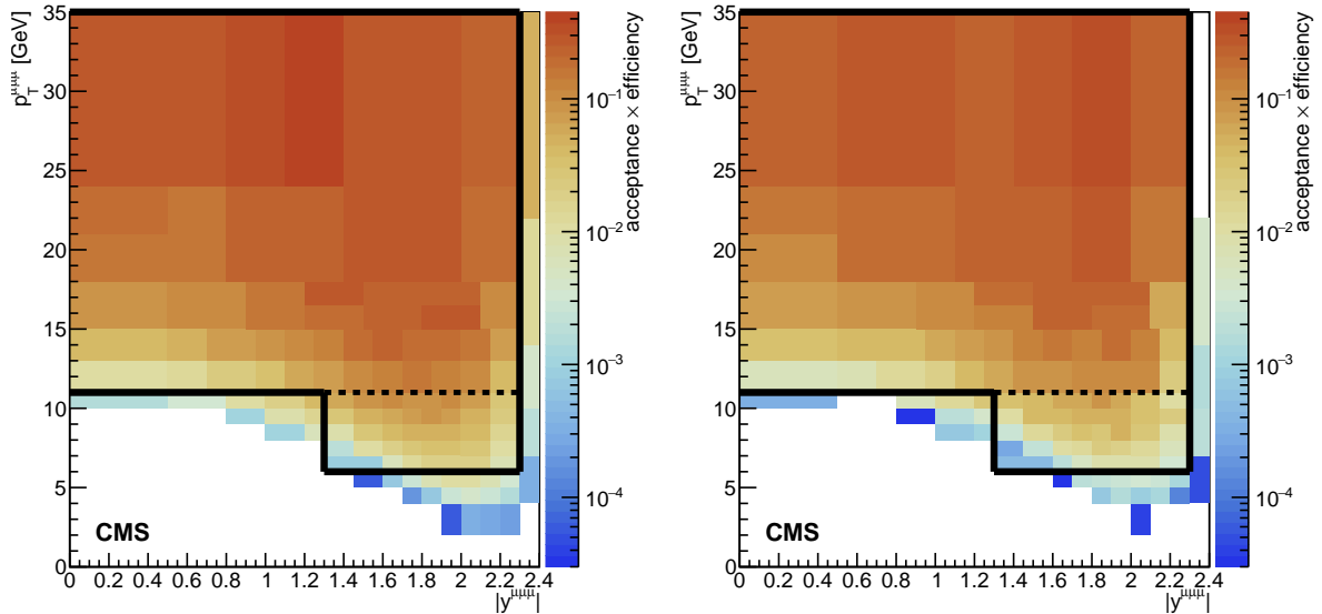
FIGURE 5.9: ( p_T^{\mu\mu\mu}, y^{\mu\mu\mu} ) map of the trimuon acceptance times efficiency (from the signal MC corrected to the final measured p_T^{\mu\mu\mu} -spectrum, see section 7.6), in pp ( left ) and PbPb ( right ). The black lines show the regions chosen as the two p_T analysis bins.
