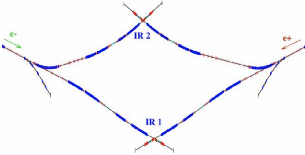
Figure 2.9: Layout of NLC Beam Delivery Systems for two IRs. Anamorphic scale (the transverse direction is stretched about a hundred times). Straight-ahead BDS for the 1 st IR and one-way-bending BDS for 2 nd IR (Figure taken from [53]).
