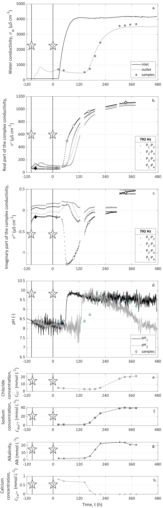
Figure 8.4: Results of Experiment ⑥. Stars 1 and 2 represent important events. Event 1 ( t = -98\text{h} ) corresponds to the injection of a non-reactive solution. Event 2 ( t = 0\text{h} ) corresponds to the beginning of the simultaneous injection of S6 and S7. (a) the inlet and outlet pore water EC measured with the in-line conductivity meters and the pore water EC of the outlet pore water samples. (b) real conductivity signal recorded on the four channels P 1 -P 2 , P 2 -P 3 , P 3 -P 4 , and P 1 -P 4 at 792 Hz. (c) imaginary conductivity signal recorded on the four channels P 1 -P 2 , P 2 -P 3 , P 3 -P 4 , and P 1 -P 4 at 127 Hz. (d) pH monitored in the column at x_{pH_1} = 13\text{ cm} and x_{pH_2} = 27\text{ cm} and pH measured on the samples of outlet pore water. (e,f,g,h) measurements of the outlet pore water chloride concentration, sodium concentration, alkalinity, and calcium concentration, respectively.
