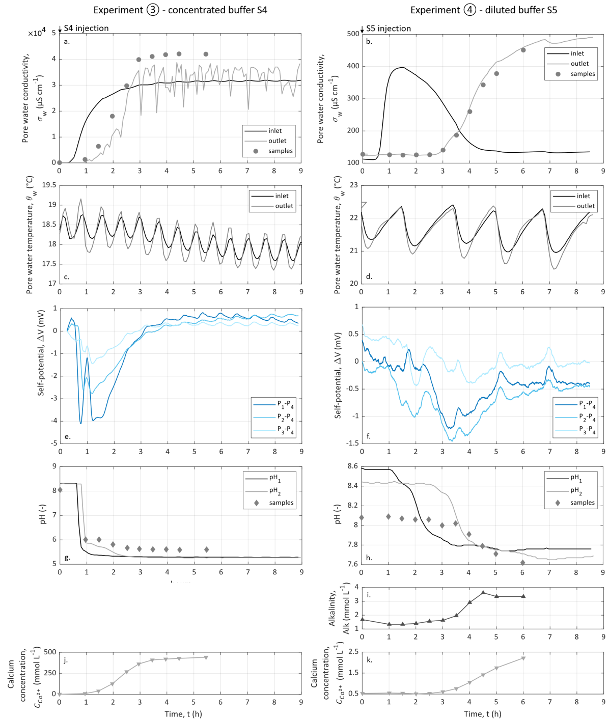
Figure 7.3: Results of experiments ③ (concentrated buffer S4) and ④ (diluted buffer S5). Injections of S4 and S5 define time-zero of each experiment. (a,b) the inlet and outlet pore water conductivity measured with the in-line conductivity meters and the pore water EC of the outlet pore water samples. (c,d) Pore water temperature monitored with the in-line conductivity meters. (e,f) SP signal recorded on three channels with electrode P_4 ( x = 23 cm) as the reference electrode. (g,h) curves of the pH monitored in the column at x_{pH_1} = 13 cm and x_{pH_2} = 27 cm and pH measured on the samples of outlet pore water. (i) alkalinity measured on the sampled outlet pore water. (j,k) calcium concentration measured on the sampled outlet pore water.
