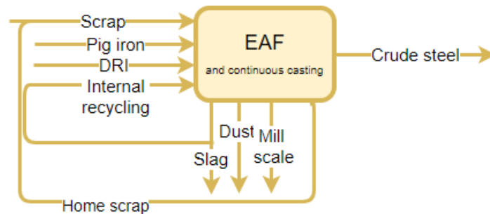
Figure 8 Flows related to the modelled EAF process
