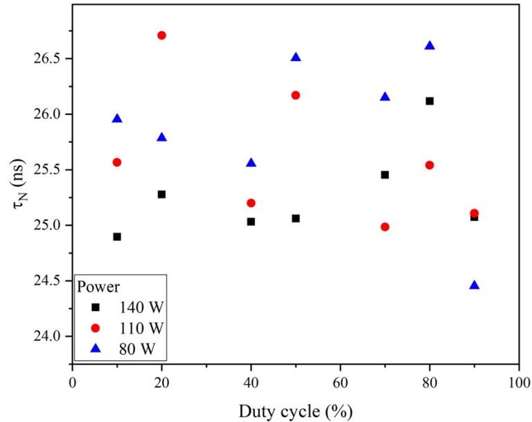
Figure 3.4: Decay time of N-atom fluorescence as a function of the duty cycle for different average input power values. The mean value of N((3p)4S^0) fluorescence decay time estimated from all these data was assessed to be 26 \pm 1.4 ns.
