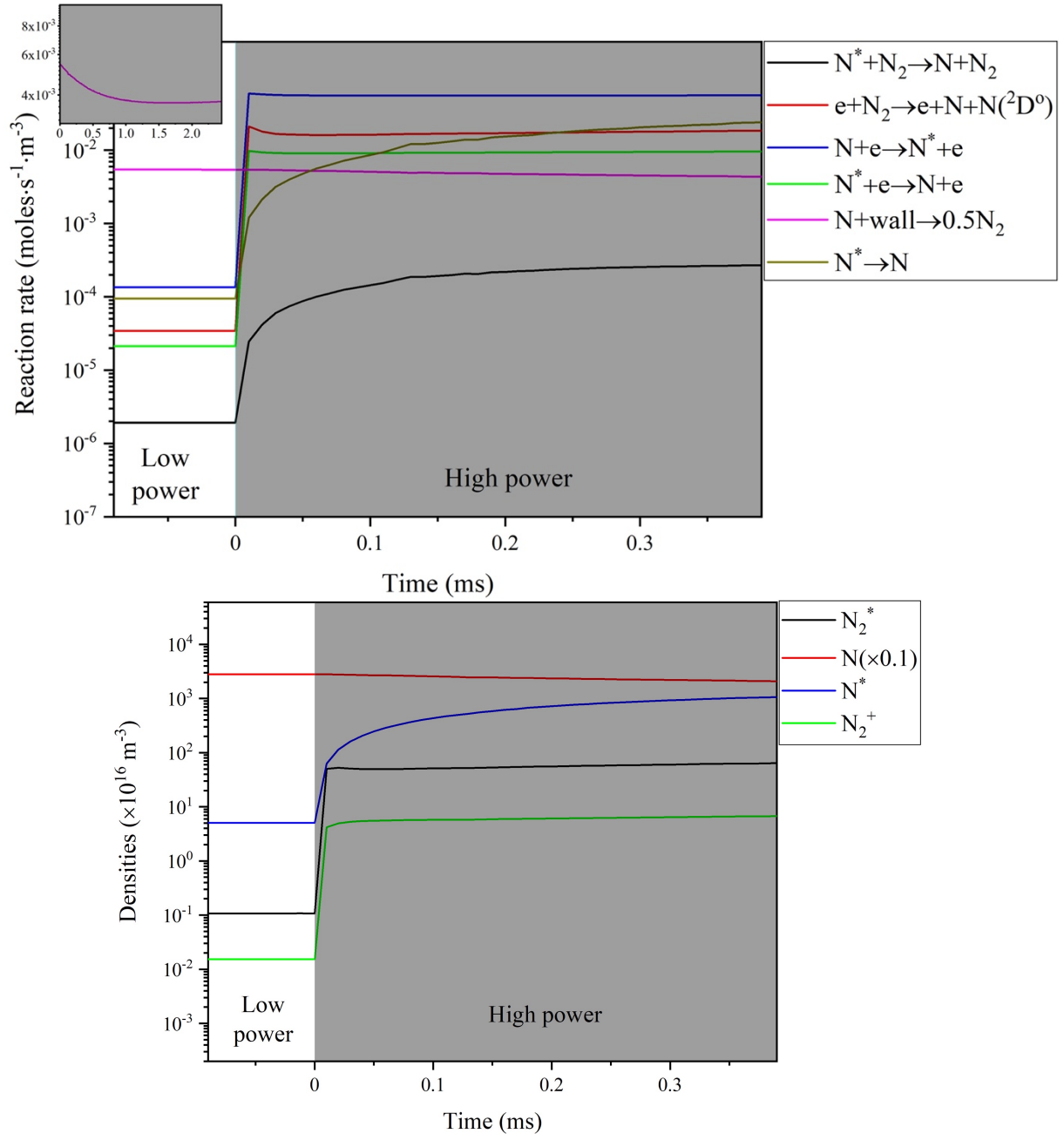
Figure 6.13: (up) Time-variation of the different processes involved in the kinetics of N(4S^0) -atom and (down) the time evolution of different species densities at the transition between the low- and high-power phases. Also shown in the insert is the increase of surface recombination of N(4S^0) in the low power phase. N_2^* and N^* indicate N_2(A^3\Sigma_u^+) and N_2(B^3\Pi_g) levels of molecular nitrogen and both considered N -atom metastable states, i.e. N(2D^0) and (2P^0) .
