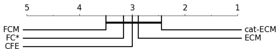
Figure B.4: Critical difference diagram obtained for FS scores with \gamma = 0.1 and \beta = 2 .
