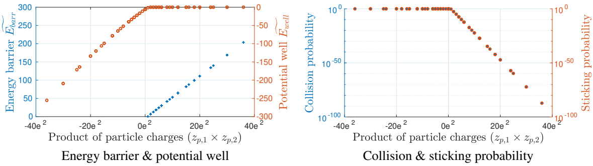
Figure 6.4: Evolution of (\widetilde{E}_{well}, \widetilde{E}_{barr}, \mathcal{P}_{coll}, \mathcal{P}_{stick}) as a function of the product of the particle electric charges. Results obtained for spherical soot particles with a size of 5 nm. The particle density and C/H ratio are obtained with variable maturity.
