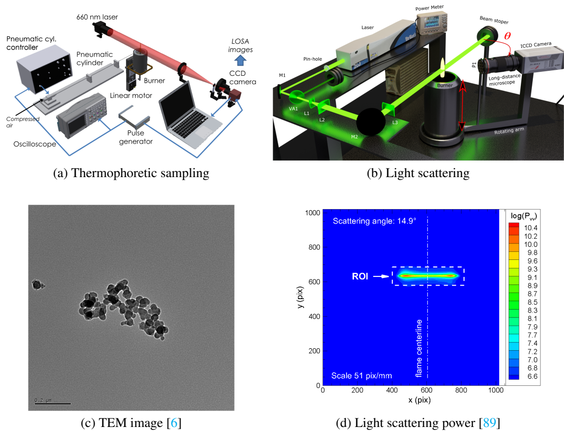
Figure 2.3: Experimental setups and examples of images (rough data) for soot aggregate characterization.
