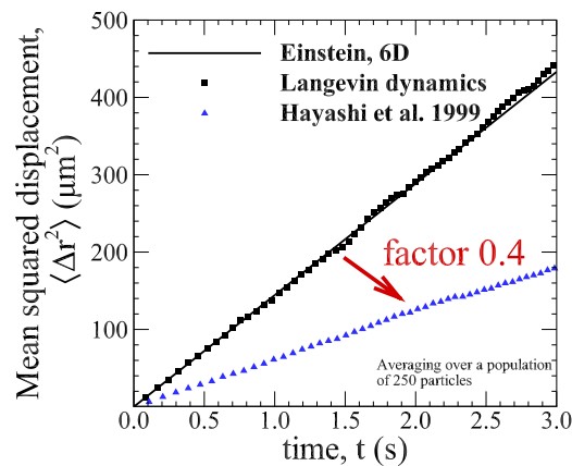
Figure 3.2: Mean squared displacement of a 1 \mu\text{m} spherical particle suspended in air at ambient conditions (fluid mean free path 66 \text{ nm} ) as a function of time. Calculated from Langevin Dynamics simulations, Einstein's theory on Brownian Motion [263] and Hayashi et al. [256] simulations.
