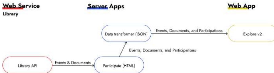
Figure 30: Back-end architecture of the second version of Explore.
