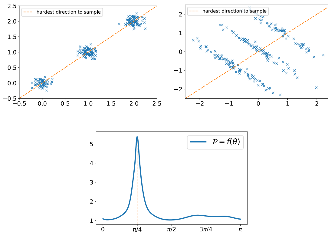
Figure 19 – (Top Left) Samples of mixture of three Gaussians. (Top right) Whiten samples of Gaussian mixture on the left. (Bottom) Plot of the Poincaré constant of the projected samples on a line of angle \theta .
