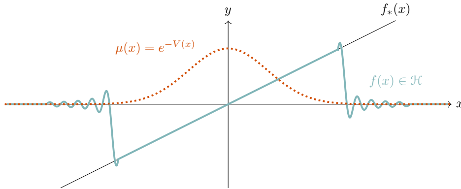
Figure 20 – Schematic figure showing the way to approximate the first eigenvector of the diffusion operator by a function in an RKHS. The example shows this in the case of a Gaussian measure in \mathbb{R} for which the first eigenfunction is the monome f_* : x \rightarrow x .
