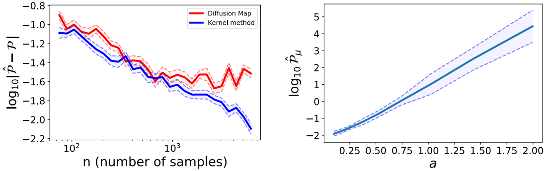
Figure 18 – (Left) Comparison of the convergences of the kernel-based method described in this paper and diffusion maps in the case of a Gaussian of variance 1 (for each n we took the mean over 50 runs). The dotted lines correspond to standard deviations of the estimator. (Right) Exponential growth of the Poincaré constant for a mixture of two Gaussians \mathcal{N}(\pm \frac{a}{2}, \sigma^2) as a function of the distance a between the two Gaussians ( \sigma = 0.1 and n = 500 ).
