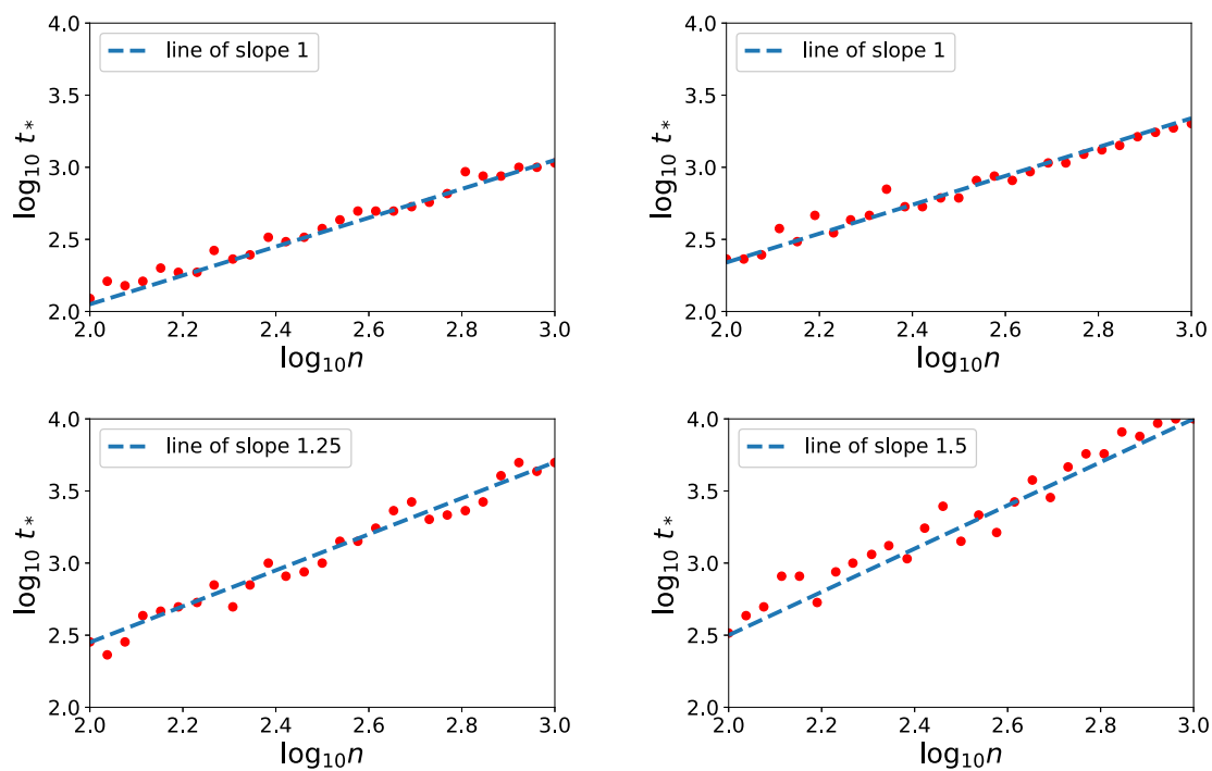
Figure 17 – The sampling is performed without replacement . The four plots represent each a different configuration on the (\alpha, r) plan represented in Figure 13, for r = 1/(2\alpha) . Top left ( \alpha = 1.5 ) and right ( \alpha = 2 ) are two easy problems (Top right is the limiting case where r = \frac{\alpha-1}{2\alpha} ) for which one pass over the data is optimal. Bottom left ( \alpha = 2.5 ) and right ( \alpha = 3 ) are two hard problems for which an increasing number of passes is required. The blue dotted line are the slopes predicted by the theoretical result in Theorem 8.
