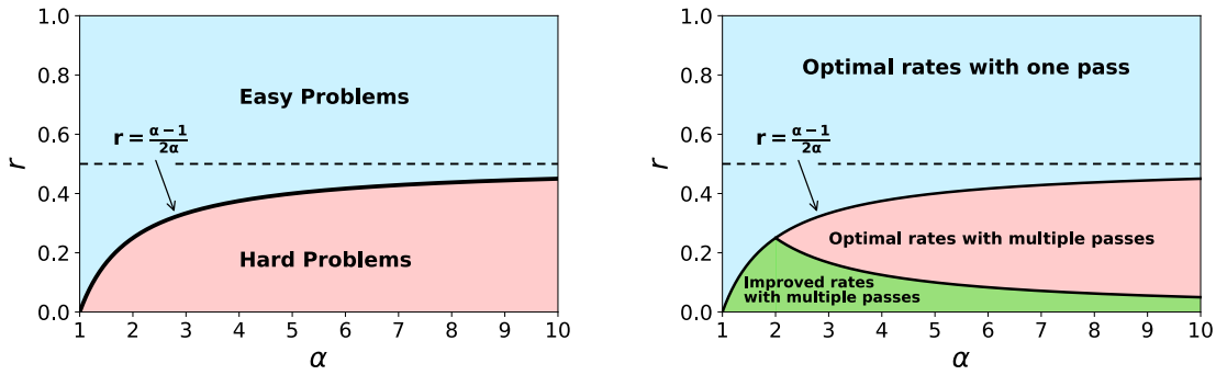
Figure 13 – (Left) easy and hard problems in the (\alpha, r) -plane. (Right) different regions for which multiple passes improved known previous bounds (green region) or reaches optimality (red region).
