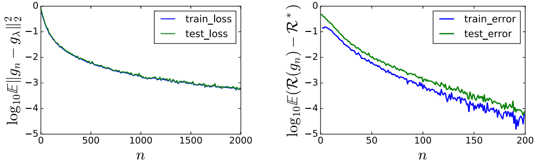
Figure 10 – Showing linear convergence for the L^{01} errors in the case of margin of width \varepsilon . Left figure corresponds to the test and training loss in the averaged case whereas the right one corresponds to the error in the same setting. Note that the y-axis is the same while the x-axis is different of a factor 10. The fact that the error plot is a line after a certain n matches our theoretical results. We took the following parameters : \varepsilon = 0.05, \gamma = 0.25, \lambda = 0.01 .
