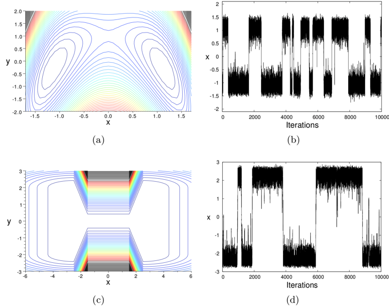
Figure 8 – (a,c) Level sets of the two-dimensional potentials in the cases of (a) energetic barrier (c) entropic barrier. (b, d) Evolution along the x -axis of the overdamped Langevin diffusion in these potentials. This figure is extracted from [LS16].
