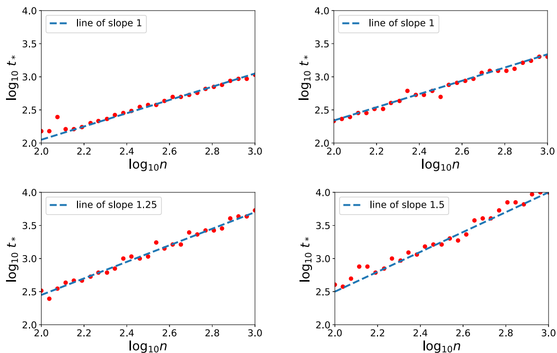
Figure 16 – The sampling is performed by cycling over the data . The four plots represent each a different configuration on the (\alpha, r) plan represented in Figure 13, for r = 1/(2\alpha) . Top left ( \alpha = 1.5 ) and right ( \alpha = 2 ) are two easy problems (Top right is the limiting case where r = \frac{\alpha-1}{2\alpha} ) for which one pass over the data is optimal. Bottom left ( \alpha = 2.5 ) and right ( \alpha = 3 ) are two hard problems for which an increasing number of passes is required. The blue dotted line are the slopes predicted by the theoretical result in Theorem 8.
