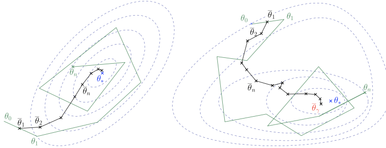
Figure 4 – Stochastic Gradient Descent with constant learning rate. Dashed lines are the level lines of the objective function f , green points correspond to the main recursion, and black to the averaged one. (Left) Quadratic case, the limit is the optimal point \theta_* . (Right) General case, the limit is a different point \bar{\theta}_\gamma at distance \gamma^2 from \theta_* .
