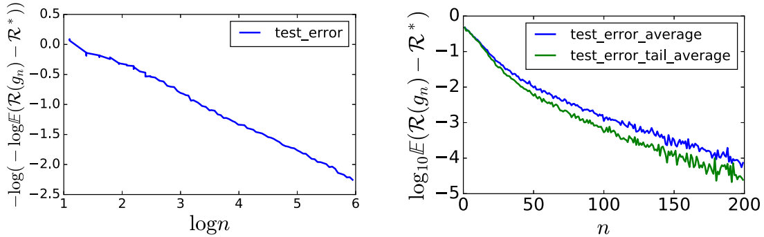
Figure 11 – Left plot shows the error in the non-averaged case for \gamma_n = \gamma/\sqrt{n} and right compares the test error between averaged and tail averaged case. We took the following parameters : \varepsilon = 0.05, \gamma = 0.25, \lambda = 0.01 .
