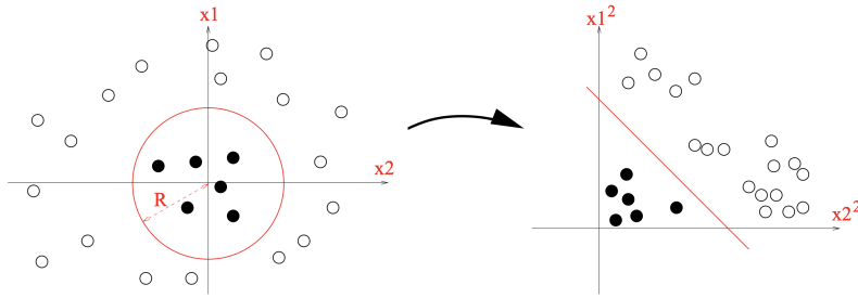
Figure 7 – Representation of the feature that maps in the case of order 2 polynomial RKHS in 2-d. We see that in the feature space the data points are linearly separated. Once again, this representation is taken from the slides of J.-P. Vert and J. Mairal lessons on Kernel methods.
