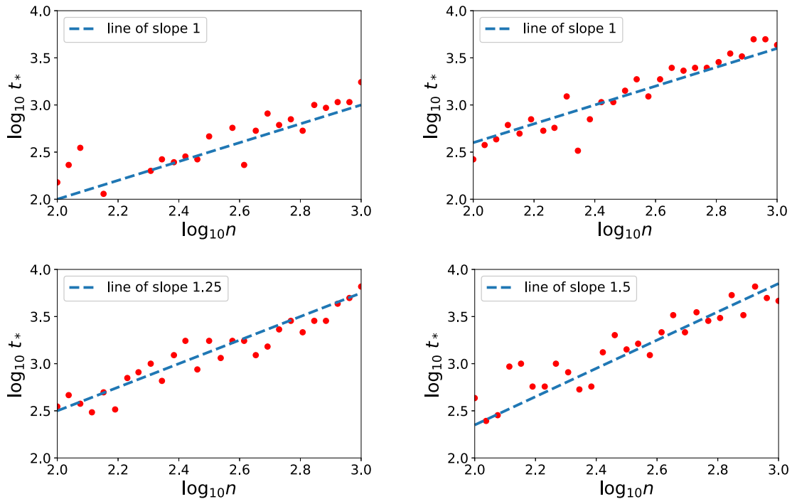
Figure 14 – The four plots represent each a different configuration on the (\alpha, r) plan represented in Figure 13, for r = 1/(2\alpha) . Top left ( \alpha = 1.5 ) and right ( \alpha = 2 ) are two easy problems (Top right is the limiting case where r = \frac{\alpha-1}{2\alpha} ) for which one pass over the data is optimal. Bottom left ( \alpha = 2.5 ) and right ( \alpha = 3 ) are two hard problems for which an increasing number of passes is required. The blue dotted line are the slopes predicted by the theoretical result in Theorem 8.
