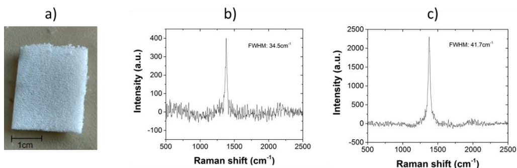
Figure 52: a) image of a 3DBN foam. b) and c) Raman spectrum of the 3DBN foam on two different points
