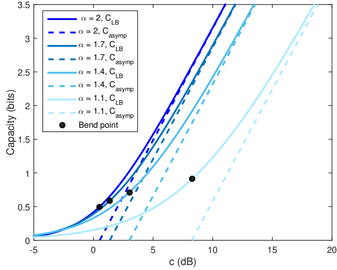
FIGURE 3.6: Plot of our capacity lower bound, C_{LB} for varying \alpha , with \gamma_N = 1 , \beta = 0 and \delta_N = 0 . The dot on each curve is the corresponding bend point.
