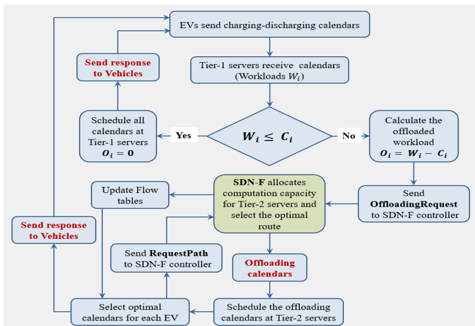
Figure 9.11- Offloading process diagram based on SDN-F controller
