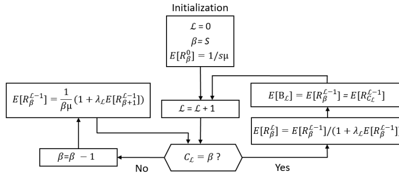
Figure 3.10 Flow Chart for Computing Mean First Passage Times and Mean Queue Move up Times
