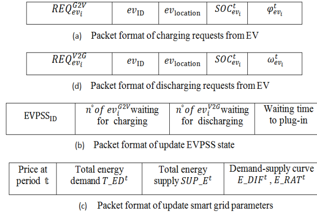
Figure 3.5- Packet format of EVs, EVSS and smart grid communications
