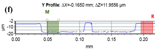
Figure 2.38 Laser interferometer estimation of the membrane curvature height and cavity depth after (a-c) XeF 2 and (d-f) HF etching. The top row shows the depth colour plots, the second (curvature estimation) and the third (cavity depth estimation) rows are \Delta Z profiles vs. the distances along the lines indicated in the colour plots.
