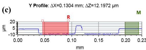
Figure 2.38 Laser interferometer estimation of the membrane curvature height and cavity depth after (a-c) XeF 2 and (d-f) HF etching. The top row shows the depth colour plots, the second (curvature estimation) and the third (cavity depth estimation) rows are \Delta Z profiles vs. the distances along the lines indicated in the colour plots.
