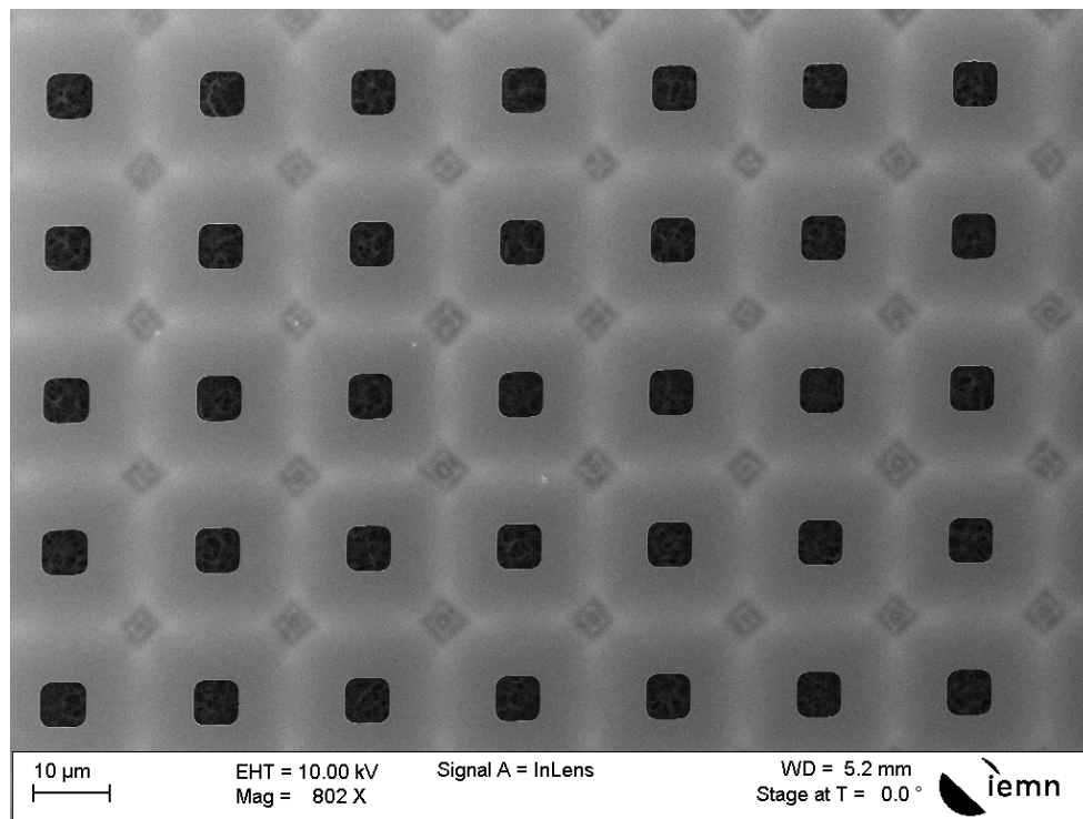
Figure 4.14 SEM image after membrane suspension from silicon substrate. The lighter out border is the result of XeF_2 etching, while the inner border represents the remaining SiO_2 after HF vapor etching.
