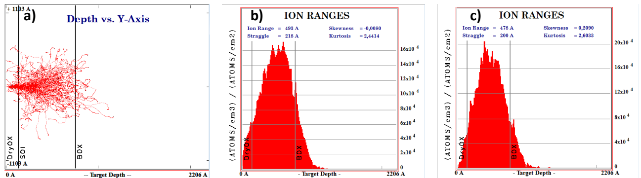
Figure 3- 24: Boron and phosphorous implantation simulation of a silicon layer. Ions propagation into the target stack (a), Ions distribution for a Boron dopant (b) and phosphorous dopant (c)
