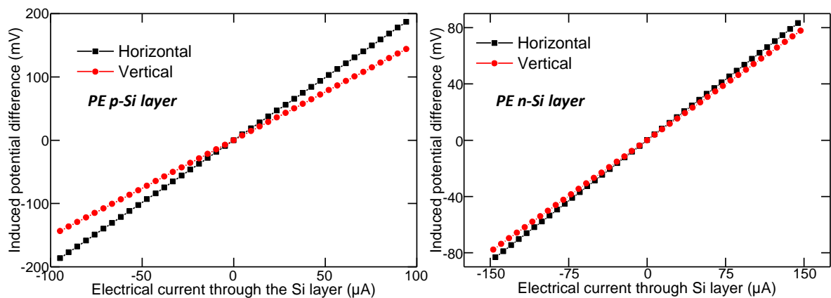
Figure 4- 8: Phonon-engineered p-Si (left) and n-Si (right) layers' electrical resistances
