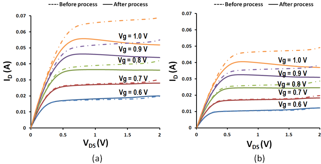
Fig. 5.9: Self heating of RF switch seen in DC characterization on TR-SOI (a) 180 nm (b) 220 nm
