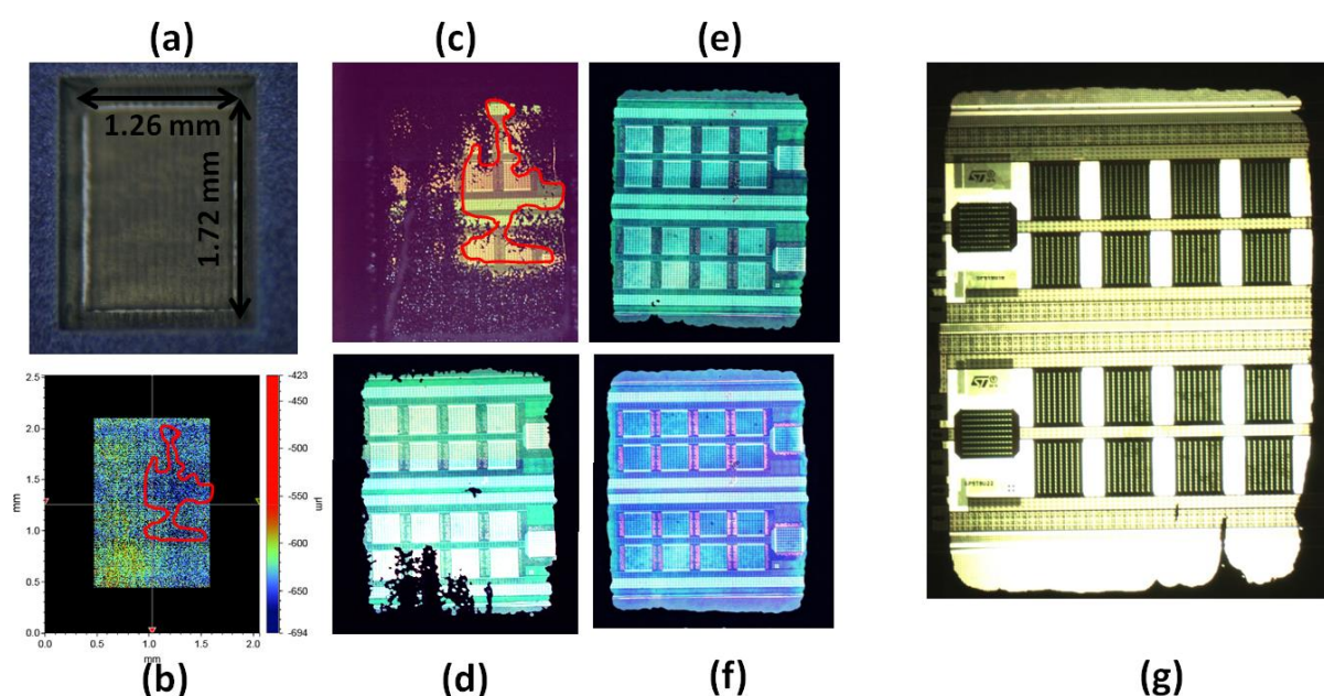
Fig. 5.7: (a) Optical micrograph of switch cavity after laser ablation (b) Profilometer scan of the ablated area with outlined region showing locally deep regions (c) After 25 cycles of XeF 2 etch. Outlined area etched first suggesting a uniform vertical etch rate of cavity (d) After 50 cycles of XeF 2 etch (e) After 75 cycles of XeF 2 etch (f) After 100 cycles of XeF 2 etch (g) View of the switch front side using backlight illumination from the cavity side.
