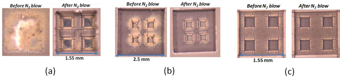
Fig. 4.22: Generation of particles during milling on 1030 nm source: (a) Case 1: Narrow opening, deep cavity (b) Case 2: Wide opening, deep cavity (c) Case 3: Narrow opening, shallow cavity. Large cavity milling parameters: Scan Speed - 50 \text{mm s}^{-1} , Fluence - 61.5 \text{J cm}^{-2} , No. of scans- 12. Small cavity milling parameters: Scan speed - 10 \text{mm s}^{-1} , Fluence - 7.1 \text{J cm}^{-2} , No. of scans - 80
