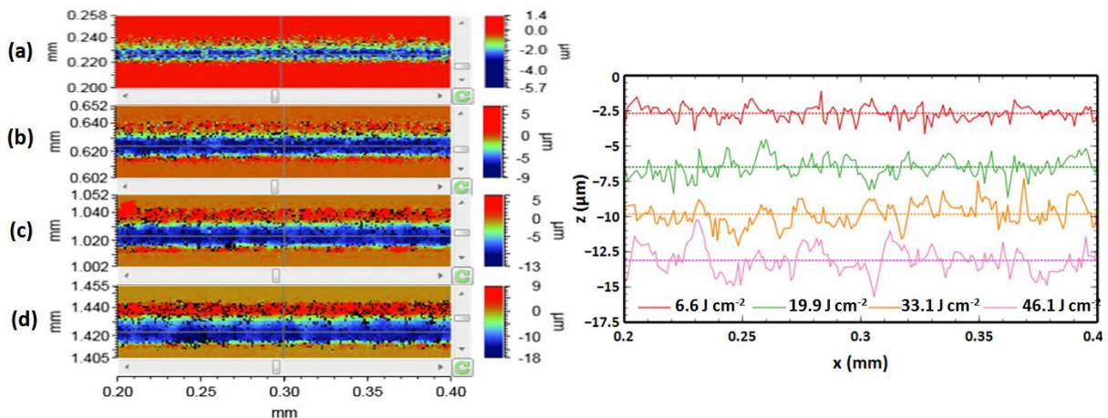
Fig. 4.11: Profile of trenches along the centre of the trench for 1030 nm source at scan speed of 30 mm s -1 repetition rate 30 kHz and fluence of (a) 6.6 J cm -2 (b) 19.9 J cm -2 (c) 33.1 J cm -2 (d) 46.1 J cm -2
