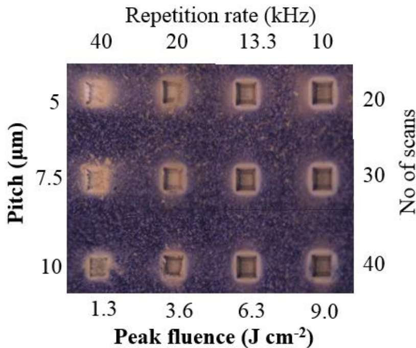
Fig. 4.21: Particle generation and redeposition as a function of laser fluence and pitch. Milling parameters (i) Source: 1030 nm (i) Area: 0.25 \times 0.25 \text{ mm}^2 (ii) Power: Column 1: 0.054 W, Column 2: 0.072 W, Column 3: 0.085 W, Column 4: 0.09 W (iii) Scan speed: 10 \text{ mm s}^{-1}
