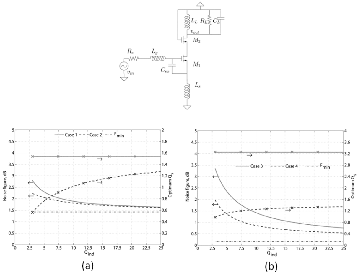
Fig. 2.23: Effect of gate inductor quality factor on noise performance for (a) Constrained gain (b) Constrained power optimization [22]
