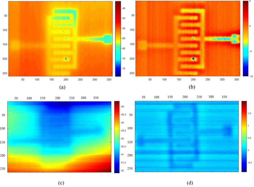
Figure II-20: The acquired image from the fabricated accelerometer on wafer: (a) The raw image with the cover layer of 2 \mu\text{m} (b) The treated image with the cover layer of 2 \mu\text{m} (c) The raw image with the cover layer of 12 \mu\text{m} (d) The treated image with the cover layer of 12 \mu\text{m} .
