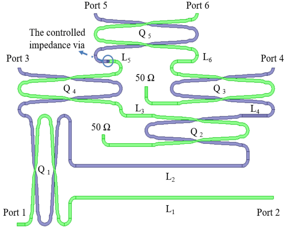
Figure IV-24: Six-port reflectometer layout based on five couplers and a controlled impedance via (The layout size is 13 cm*10 cm).
