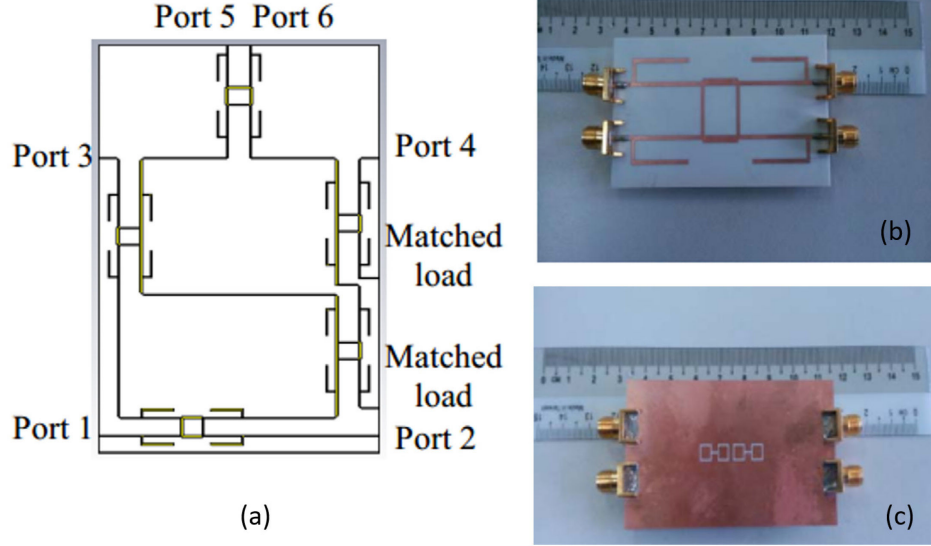
Figure IV-4: The six-port reflectometer with five branch line couplers (a) The layout of branch line coupler (b) Top view of branch line coupler (c) Bottom view of branch line coupler using defect ground structure technique (DGS) [SHU 14].
