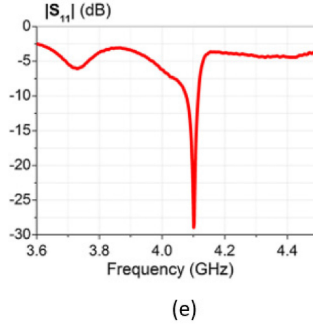
Figure I-9: Schematic of four typical resonator based matching networks and an example of a measured reflection coefficient: (a) a split-ring resonator [REN 11] (b) a resonant waveguide [KIM 04] (c) a loaded aperture probe [MAL 16] (d) a coaxial resonator [WAN 07] (e) The measured reflection coefficient in terms of magnitude at the resonance frequency (4.1 GHz) for the resonant waveguide [KIM 04].
