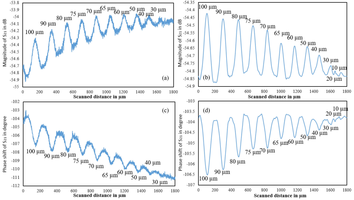
Figure II-15: Measured magnitude and phase shift of the transmission coefficient S_{21} , Zero level = -55 dB, F = 18 GHz, H = 1 \mu m, EMP= 30 \mu m (a) raw data in magnitude (b) balanced and denoised data in magnitude (c) raw data for phase shift (d) balanced and denoised data for phase shift.
