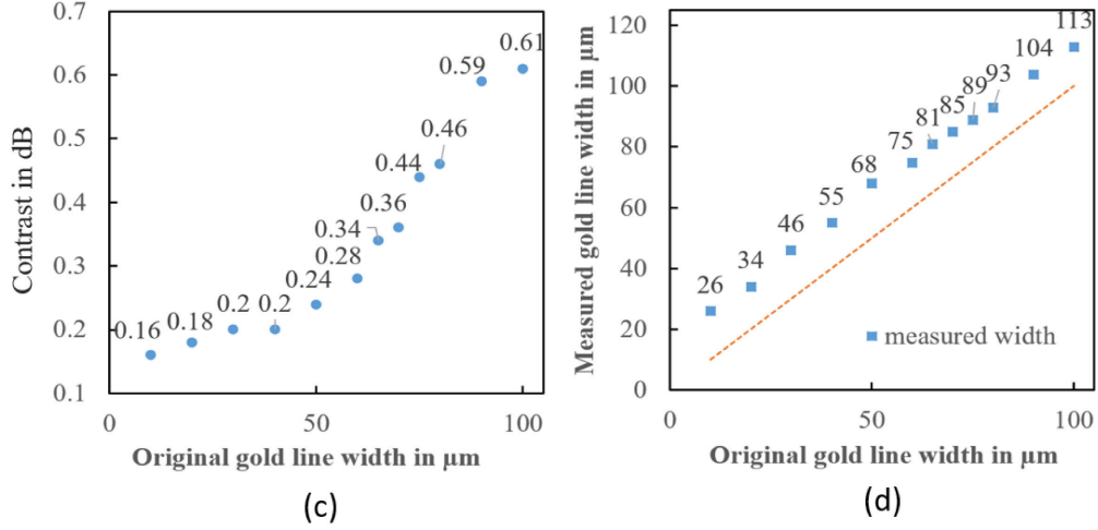
Figure II-11: (a) gold lines with various widths (b) Measured magnitude of the transmission coefficient S_{21} over a set of lines with different widths ranging from 10 to 100 \mu\text{m} , tip apex = 30 \mu\text{m} , F = 18 GHz, H = 1 \mu\text{m} (c) Measurement contrast for different gold lines (d) line width measured for each gold line compared to the original width.
