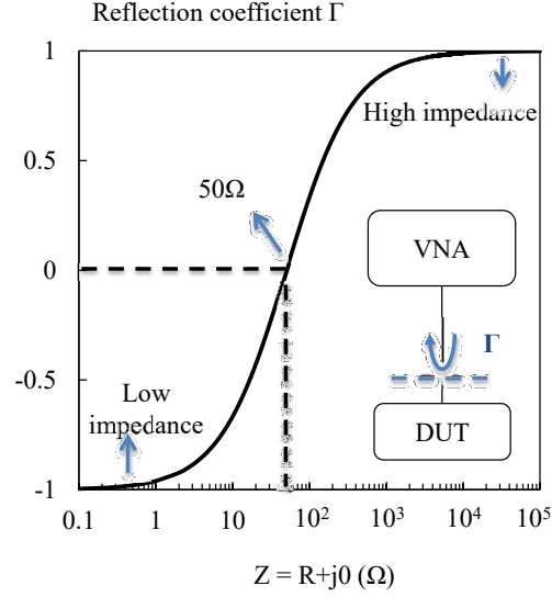
Figure I-8: Reflection coefficient \Gamma as a function of a pure resistive impedance (DUT). The VNA intrinsic impedance is 50 Ω [GU 16_c].
