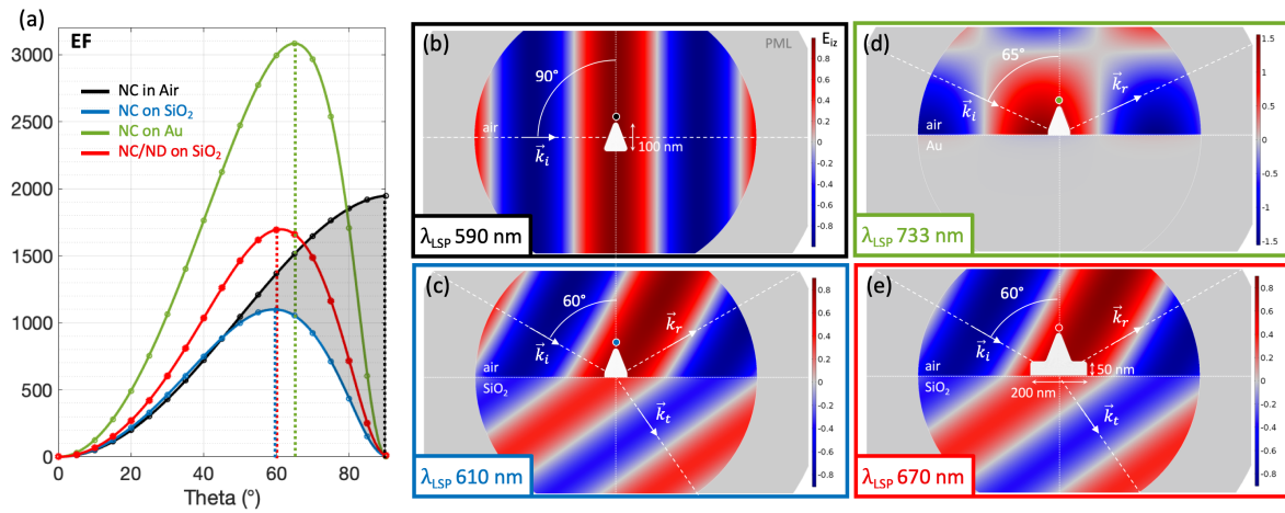
FIGURE 4.1 – (a) EF as a function of the excitation angle - at a specific excitation wavelength - for a single AuNC in air (in black - at 590nm), on \text{SiO}_2 surface (in blue - at 610nm), on a gold surface (in green - at 733nm) and a combination of AuNC-AuND on a \text{SiO}_2 surface (in red - at 670 nm). (b-e) Corresponding maps of the z-component of the incoming plane wave at the optimized value of the incident angle.
