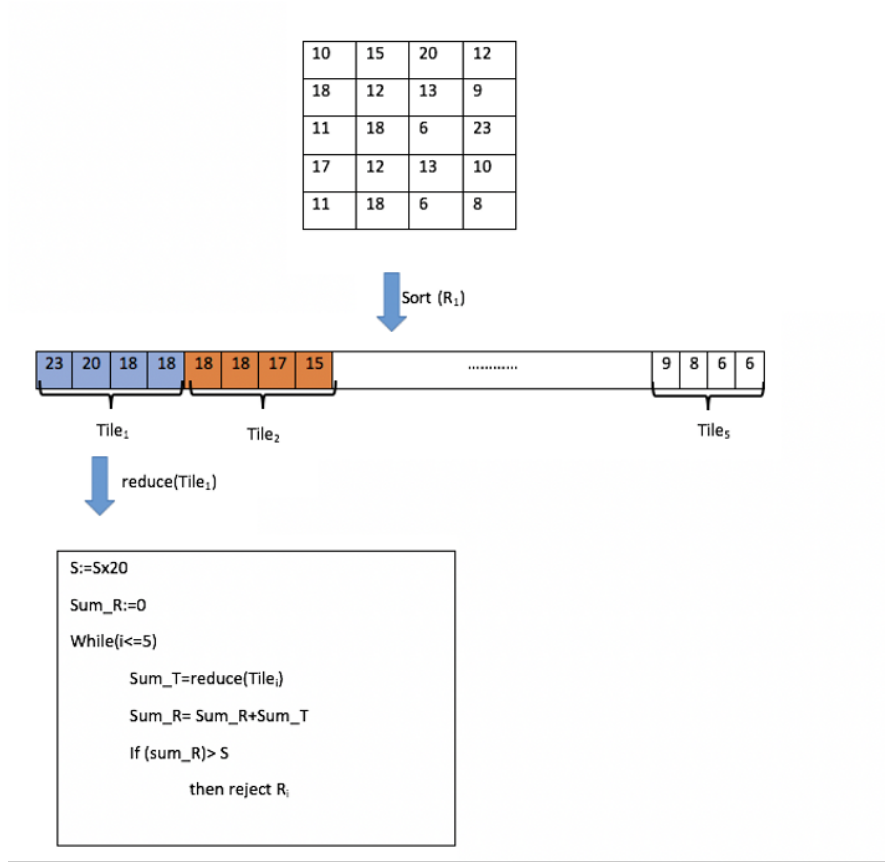
Figure 6.2. Illustration of our method for one raster( R_1 ).
