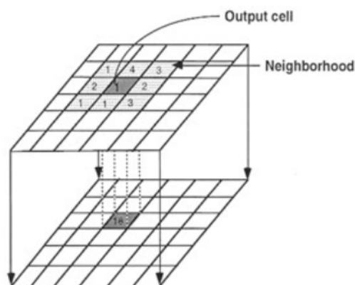
Figure 3.9. Focal functions.
