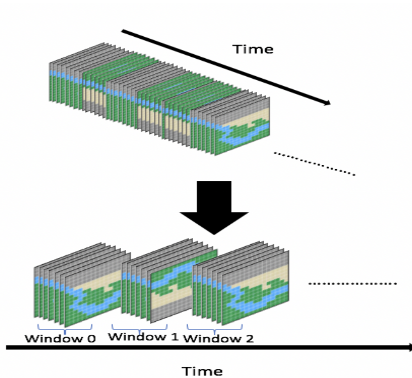
Figure 6.1. Dividing the dataset into time windows (subsequence of rasters).
